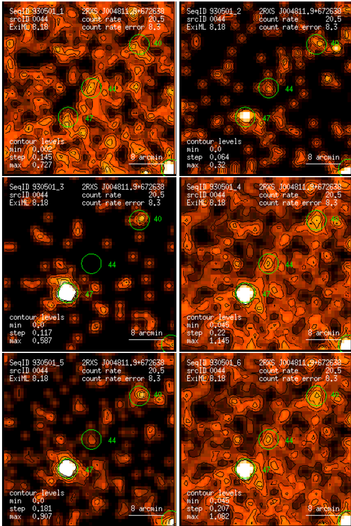
Figure 44: RASS 930501: detection 0044: band rate images, Gaussian filter: (1) PSPC channels 11 – 41, (2) 52 – 90, (3) 91 – 201, (4) 11 – 235, (5) 52 – 201, (6) 11 – 201. Broad band rates in counts/ks. Band rate contour levels in counts/ks/arcmin 2 .
