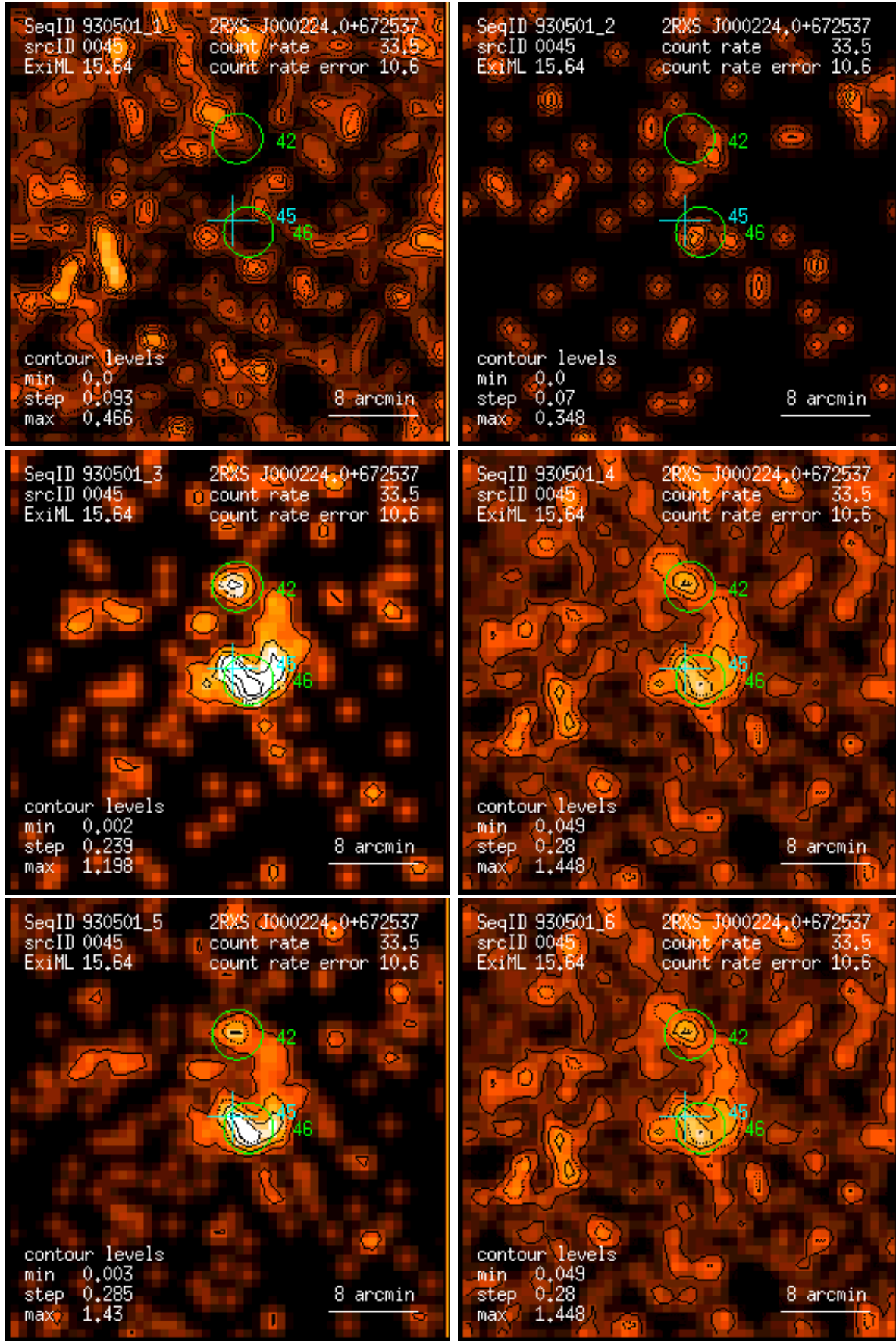
Figure 45: RASS 930501: detection 0045: band rate images, Gaussian filter: (1) PSPC channels 11 – 41, (2) 52 – 90, (3) 91 – 201, (4) 11 – 235, (5) 52 – 201, (6) 11 – 201. Broad band rates in counts/ks. Band rate contour levels in counts/ks/arcmin 2 .
