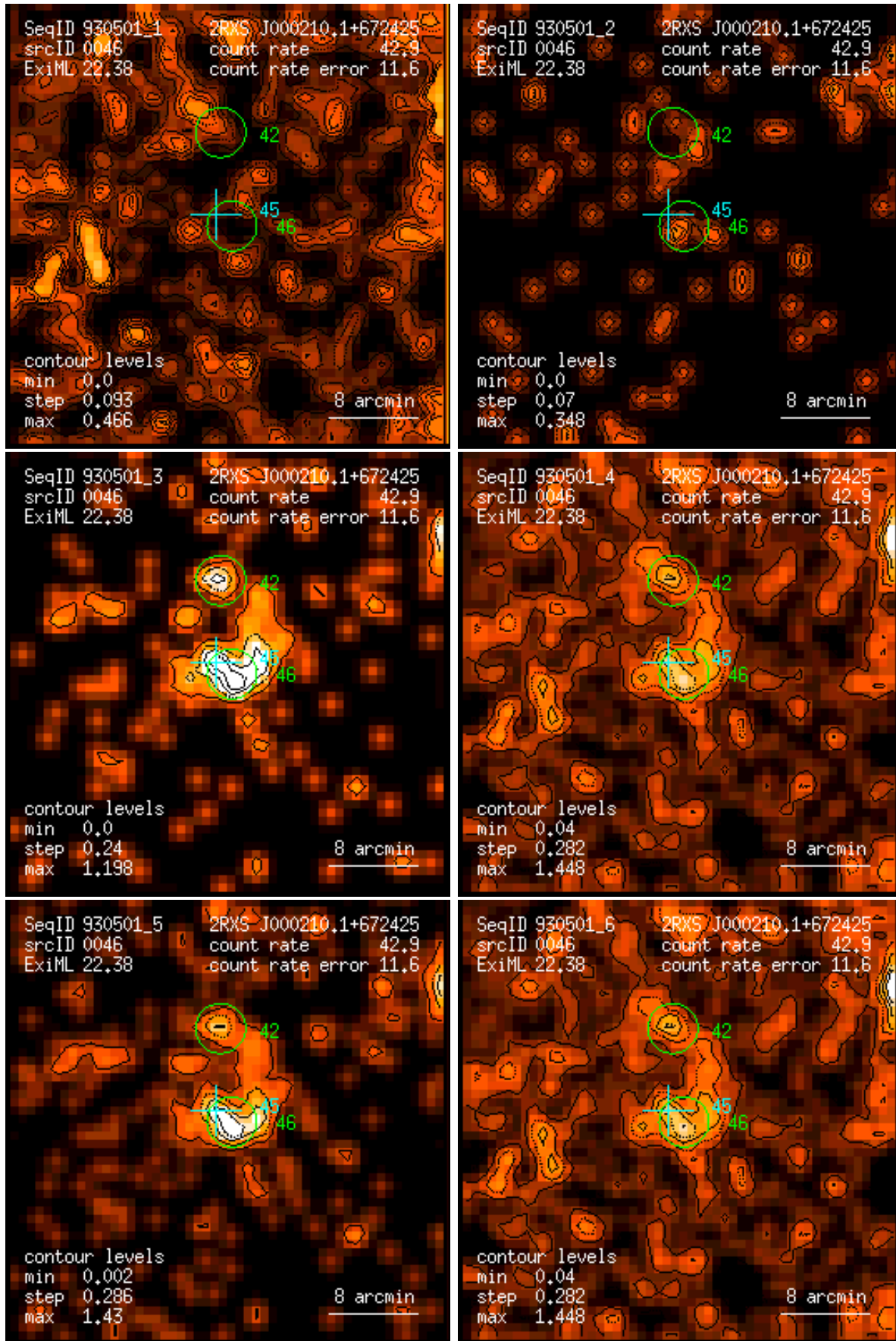
Figure 46: RASS 930501: detection 0046: band rate images, Gaussian filter: (1) PSPC channels 11 – 41, (2) 52 – 90, (3) 91 – 201, (4) 11 – 235, (5) 52 – 201, (6) 11 – 201. Broad band rates in counts/ks. Band rate contour levels in counts/ks/arcmin 2 .
