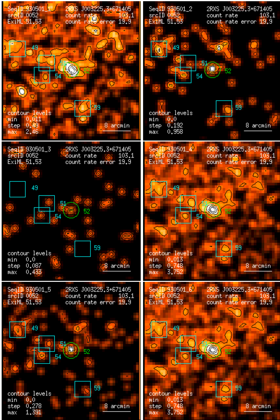
Figure 52: RASS 930501: detection 0052: band rate images, Gaussian filter: (1) PSPC channels 11 – 41, (2) 52 – 90, (3) 91 – 201, (4) 11 – 235, (5) 52 – 201, (6) 11 – 201. Broad band rates in counts/ks. Band rate contour levels in counts/ks/arcmin 2 .
