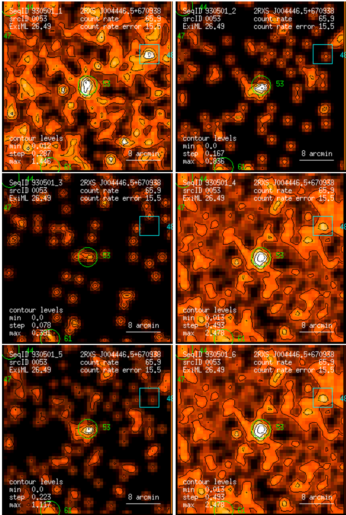
Figure 53: RASS 930501: detection 0053: band rate images, Gaussian filter: (1) PSPC channels 11 – 41, (2) 52 – 90, (3) 91 – 201, (4) 11 – 235, (5) 52 – 201, (6) 11 – 201. Broad band rates in counts/ks. Band rate contour levels in counts/ks/arcmin 2 .
