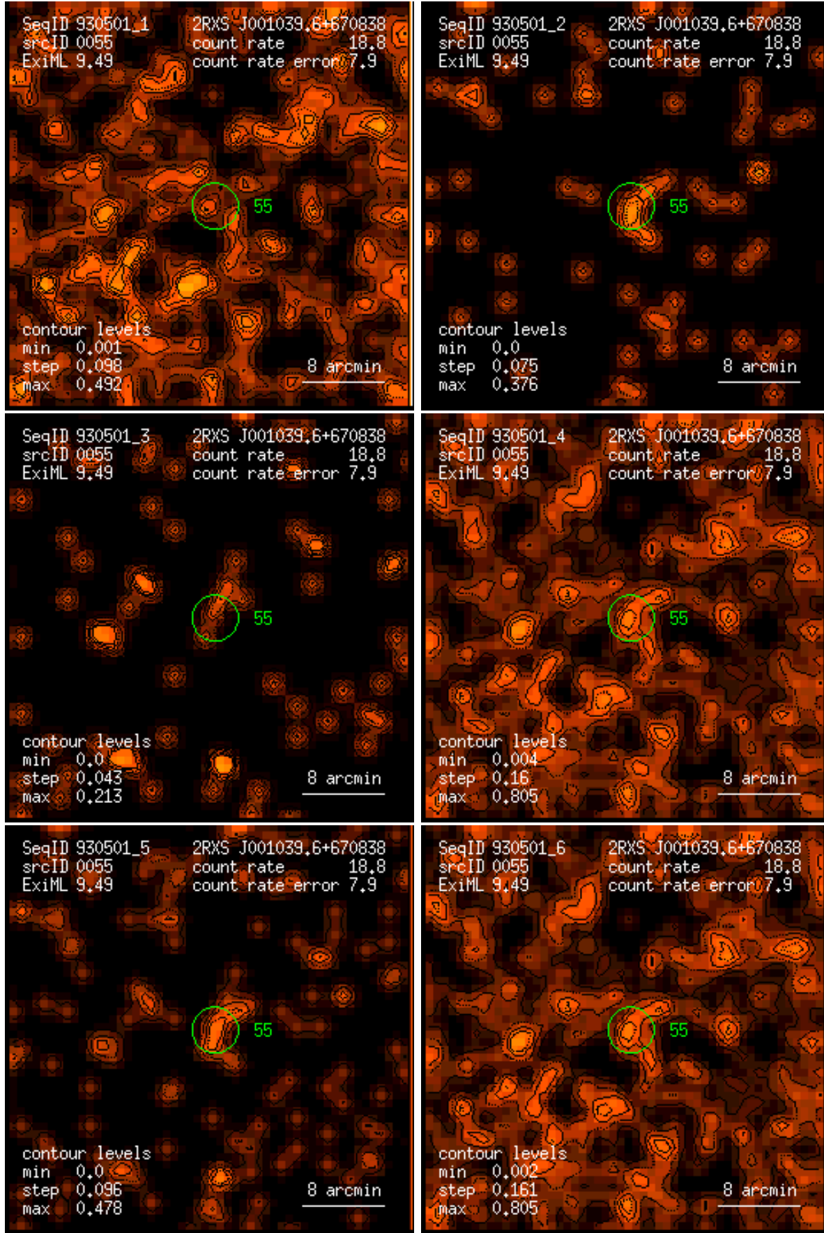
Figure 55: RASS 930501: detection 0055: band rate images, Gaussian filter: (1) PSPC channels 11 – 41, (2) 52 – 90, (3) 91 – 201, (4) 11 – 235, (5) 52 – 201, (6) 11 – 201. Broad band rates in counts/ks. Band rate contour levels in counts/ks/arcmin 2 .
