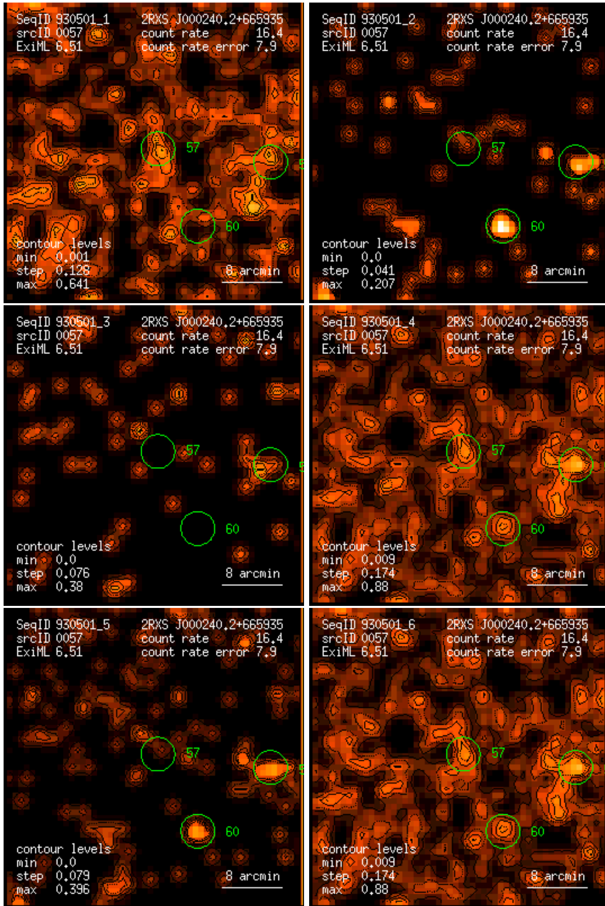
Figure 57: RASS 930501: detection 0057: band rate images, Gaussian filter: (1) PSPC channels 11 – 41, (2) 52 – 90, (3) 91 – 201, (4) 11 – 235, (5) 52 – 201, (6) 11 – 201. Broad band rates in counts/ks. Band rate contour levels in counts/ks/arcmin 2 .
