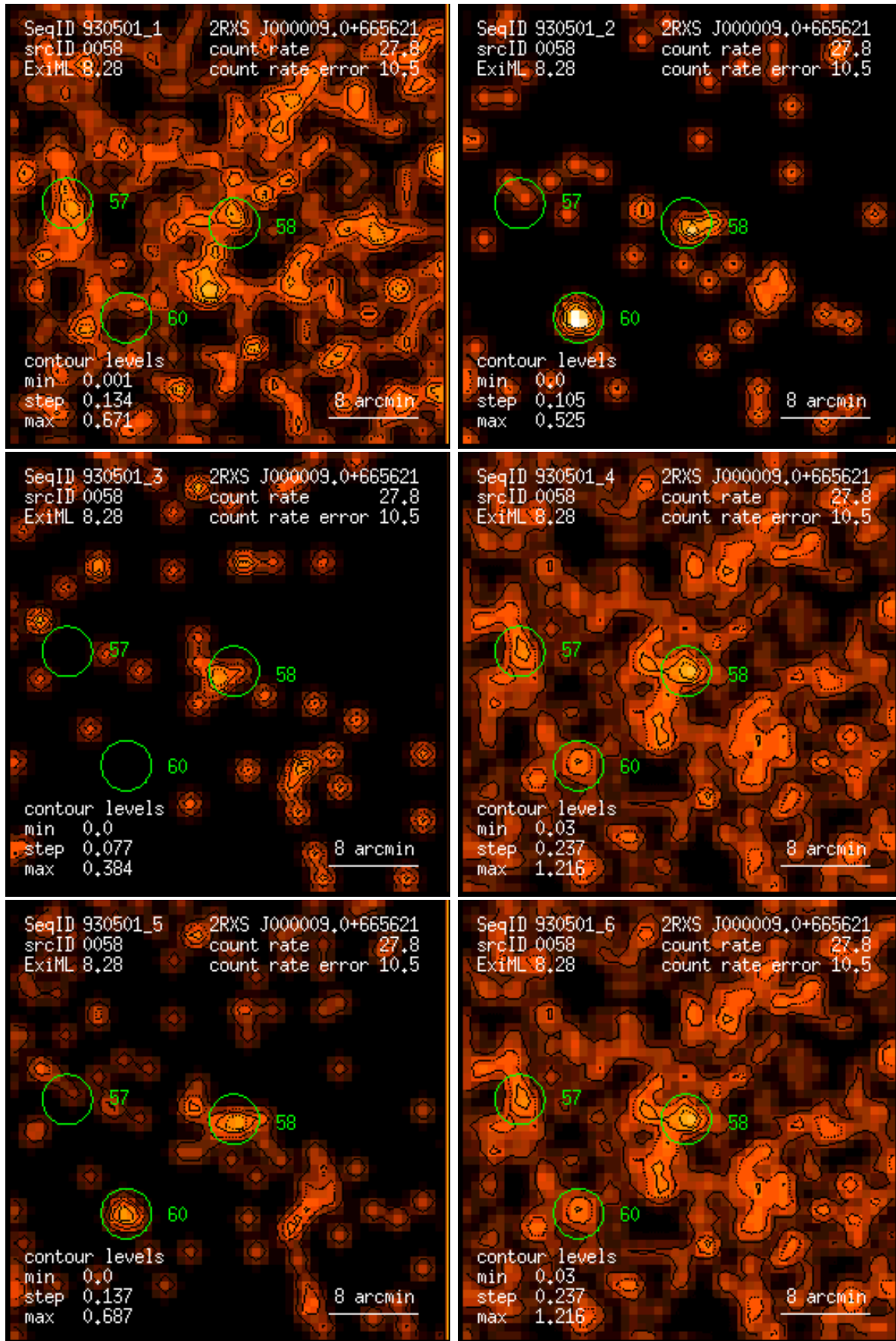
Figure 58: RASS 930501: detection 0058: band rate images, Gaussian filter: (1) PSPC channels 11 – 41, (2) 52 – 90, (3) 91 – 201, (4) 11 – 235, (5) 52 – 201, (6) 11 – 201. Broad band rates in counts/ks. Band rate contour levels in counts/ks/arcmin 2 .
