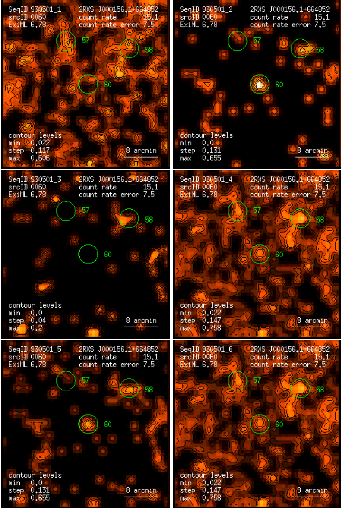
Figure 60: RASS 930501: detection 0060: band rate images, Gaussian filter: (1) PSPC channels 11 – 41, (2) 52 – 90, (3) 91 – 201, (4) 11 – 235, (5) 52 – 201, (6) 11 – 201. Broad band rates in counts/ks. Band rate contour levels in counts/ks/arcmin 2 .
