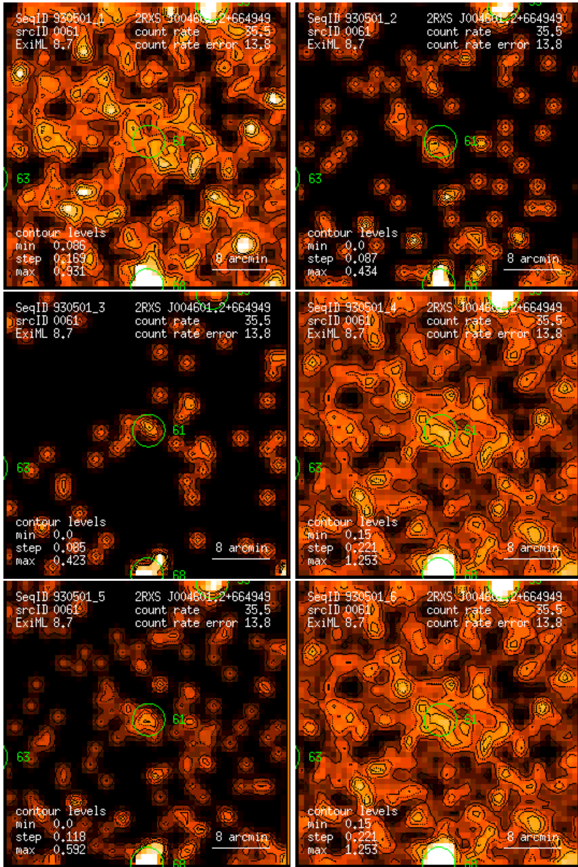
Figure 61: RASS 930501: detection 0061: band rate images, Gaussian filter: (1) PSPC channels 11 – 41, (2) 52 – 90, (3) 91 – 201, (4) 11 – 235, (5) 52 – 201, (6) 11 – 201. Broad band rates in counts/ks. Band rate contour levels in counts/ks/arcmin 2 .
