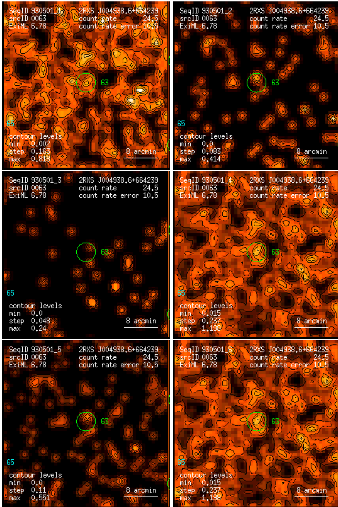
Figure 63: RASS 930501: detection 0063: band rate images, Gaussian filter: (1) PSPC channels 11 – 41, (2) 52 – 90, (3) 91 – 201, (4) 11 – 235, (5) 52 – 201, (6) 11 – 201. Broad band rates in counts/ks. Band rate contour levels in counts/ks/arcmin 2 .
