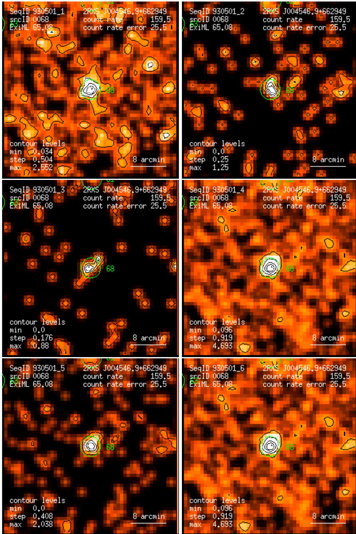
Figure 68: RASS 930501: detection 0068: band rate images, Gaussian filter: (1) PSPC channels 11 – 41, (2) 52 – 90, (3) 91 – 201, (4) 11 – 235, (5) 52 – 201, (6) 11 – 201. Broad band rates in counts/ks. Band rate contour levels in counts/ks/arcmin 2 .
