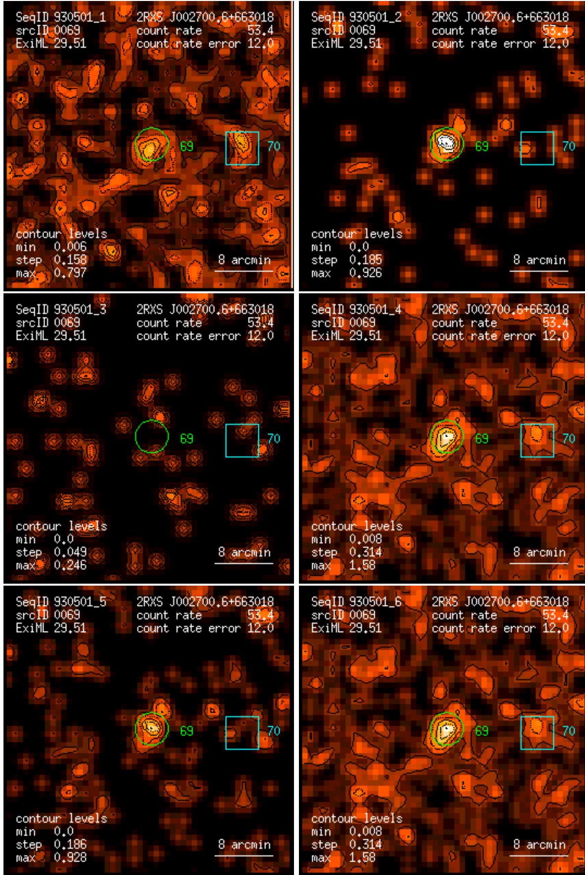
Figure 69: RASS 930501: detection 0069: band rate images, Gaussian filter: (1) PSPC channels 11 – 41, (2) 52 – 90, (3) 91 – 201, (4) 11 – 235, (5) 52 – 201, (6) 11 – 201. Broad band rates in counts/ks. Band rate contour levels in counts/ks/arcmin 2 .
