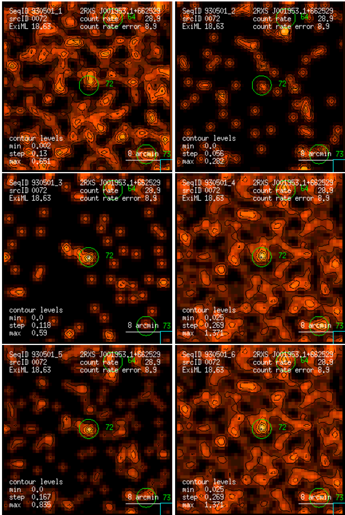
Figure 72: RASS 930501: detection 0072: band rate images, Gaussian filter: (1) PSPC channels 11 – 41, (2) 52 – 90, (3) 91 – 201, (4) 11 – 235, (5) 52 – 201, (6) 11 – 201. Broad band rates in counts/ks. Band rate contour levels in counts/ks/arcmin 2 .
