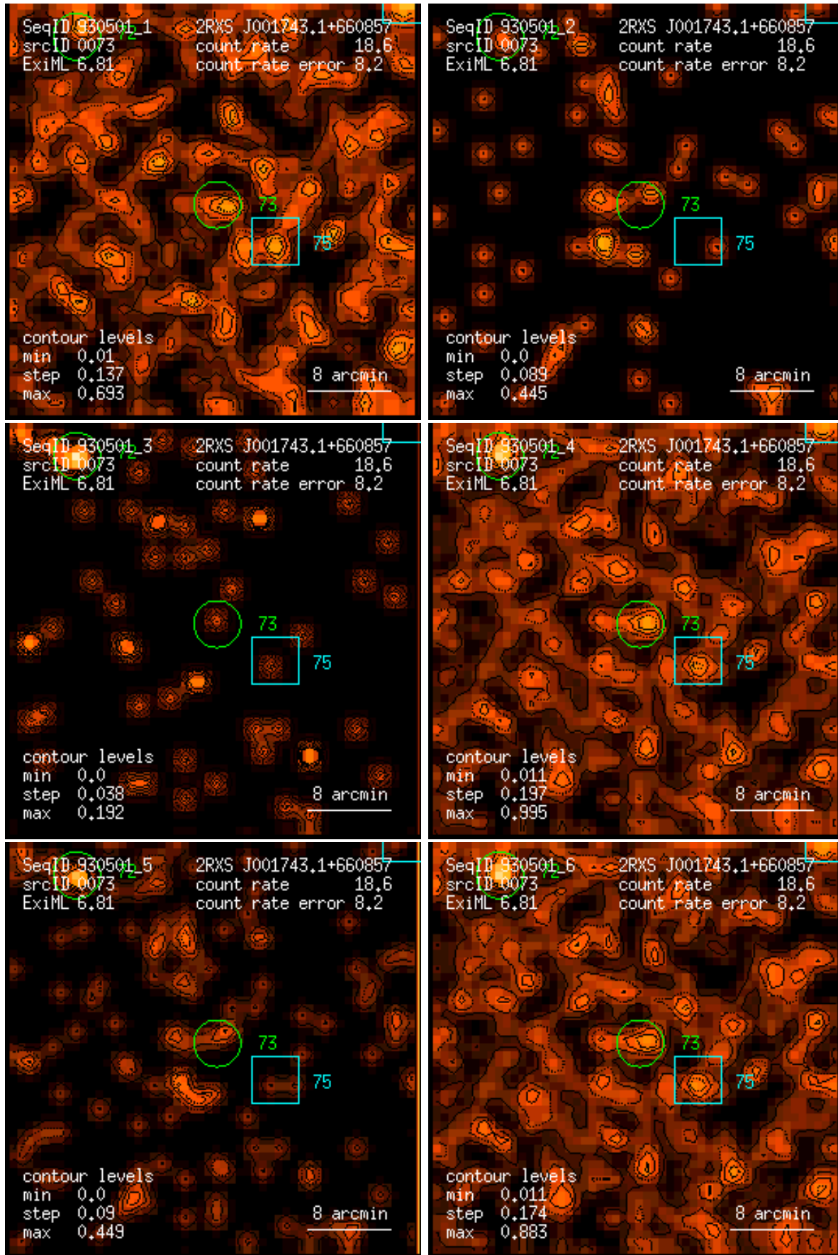
Figure 73: RASS 930501: detection 0073: band rate images, Gaussian filter: (1) PSPC channels 11 – 41, (2) 52 – 90, (3) 91 – 201, (4) 11 – 235, (5) 52 – 201, (6) 11 – 201. Broad band rates in counts/ks. Band rate contour levels in counts/ks/arcmin 2 .
