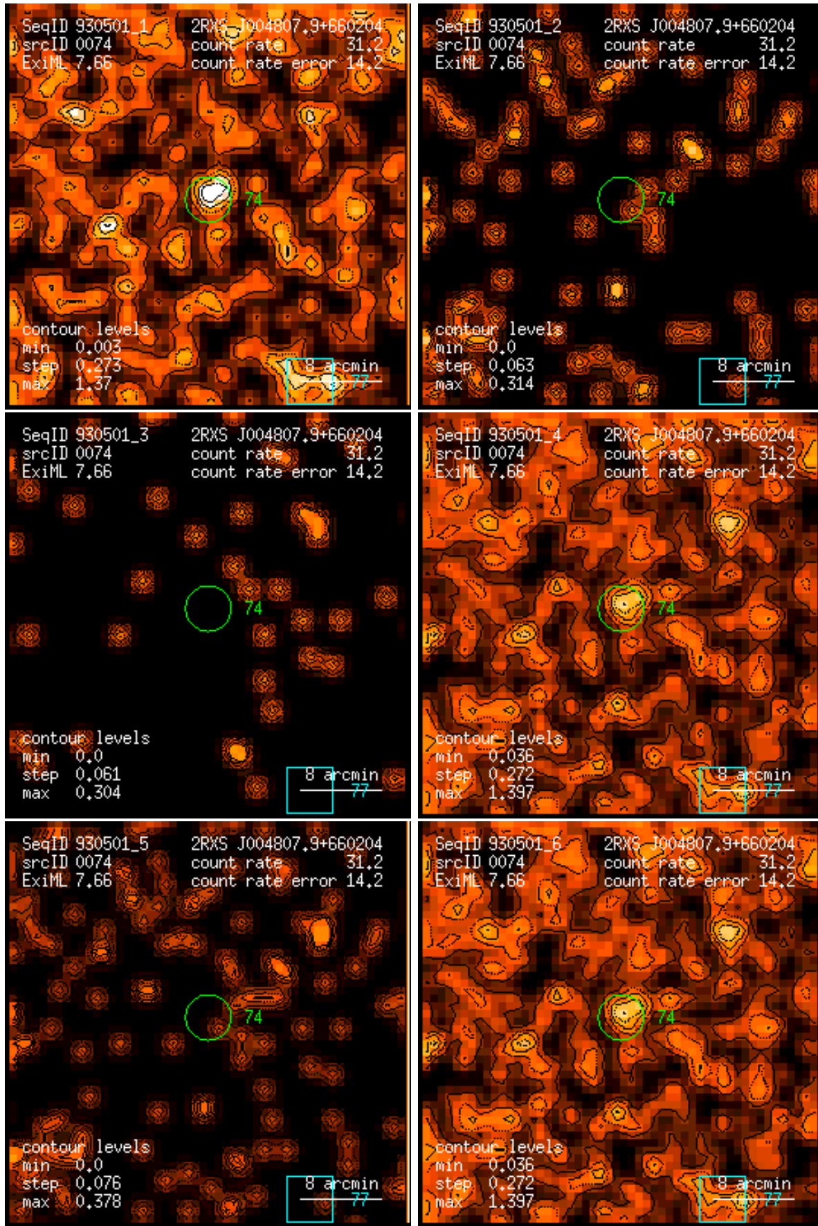
Figure 74: RASS 930501: detection 0074: band rate images, Gaussian filter: (1) PSPC channels 11 – 41, (2) 52 – 90, (3) 91 – 201, (4) 11 – 235, (5) 52 – 201, (6) 11 – 201. Broad band rates in counts/ks. Band rate contour levels in counts/ks/arcmin 2 .
