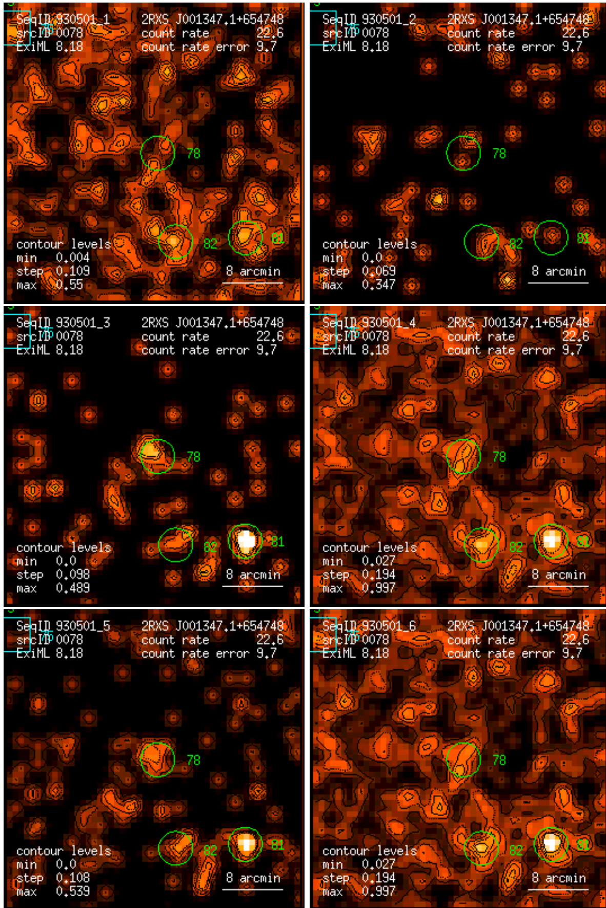
Figure 78: RASS 930501: detection 0078: band rate images, Gaussian filter: (1) PSPC channels 11 – 41, (2) 52 – 90, (3) 91 – 201, (4) 11 – 235, (5) 52 – 201, (6) 11 – 201. Broad band rates in counts/ks. Band rate contour levels in counts/ks/arcmin 2 .
