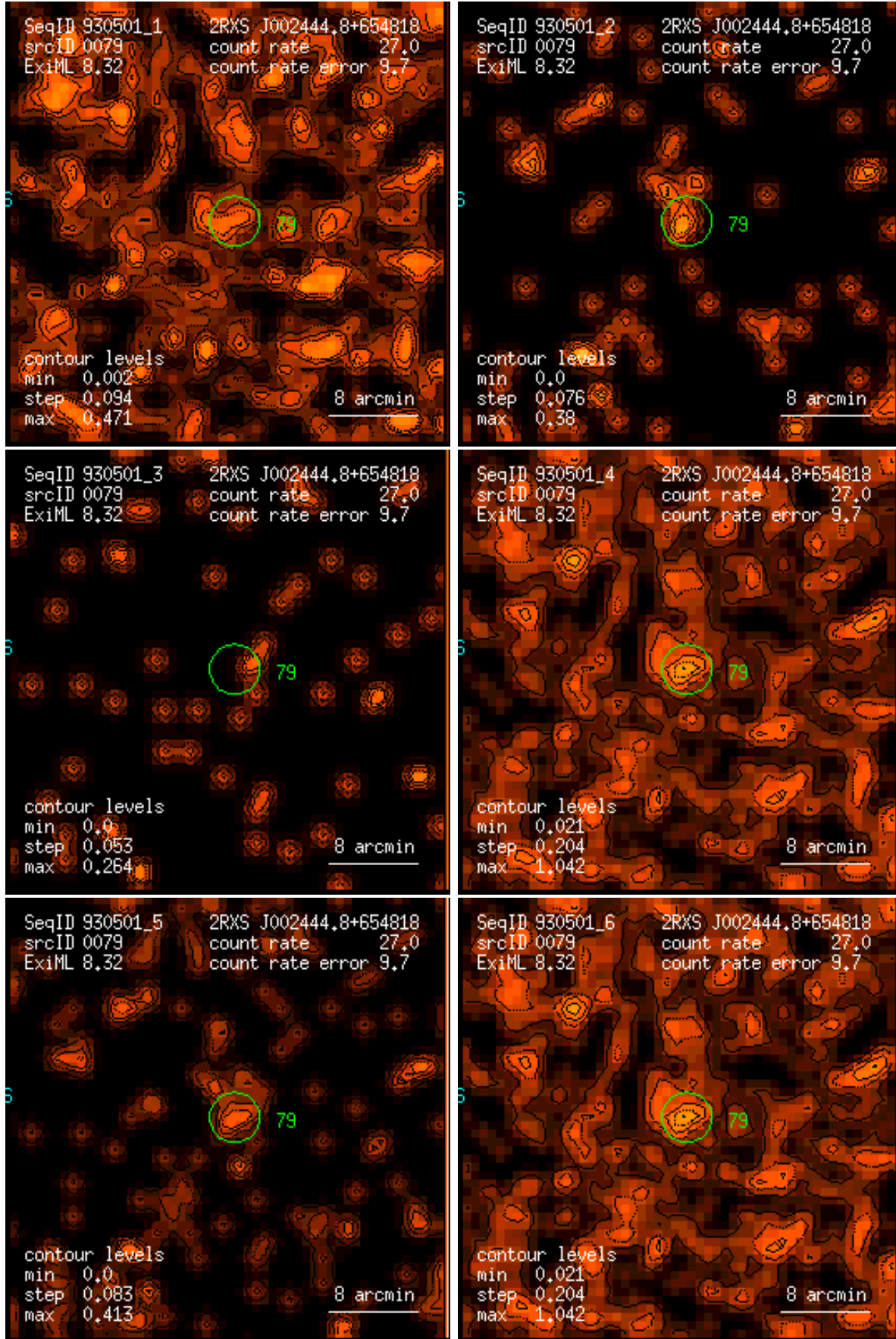
Figure 79: RASS 930501: detection 0079: band rate images, Gaussian filter: (1) PSPC channels 11 – 41, (2) 52 – 90, (3) 91 – 201, (4) 11 – 235, (5) 52 – 201, (6) 11 – 201. Broad band rates in counts/ks. Band rate contour levels in counts/ks/arcmin 2 .
