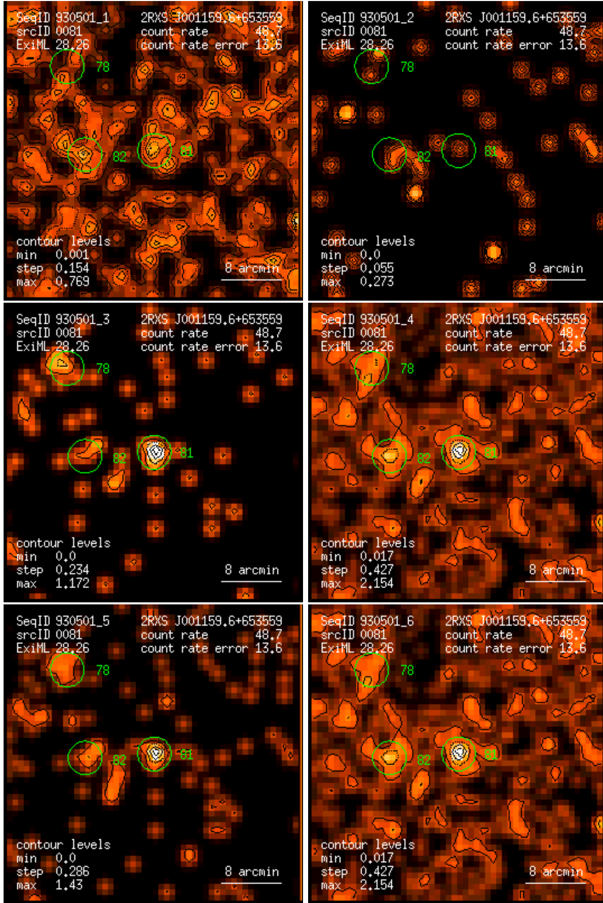
Figure 81: RASS 930501: detection 0081: band rate images, Gaussian filter: (1) PSPC channels 11 – 41, (2) 52 – 90, (3) 91 – 201, (4) 11 – 235, (5) 52 – 201, (6) 11 – 201. Broad band rates in counts/ks. Band rate contour levels in counts/ks/arcmin 2 .
