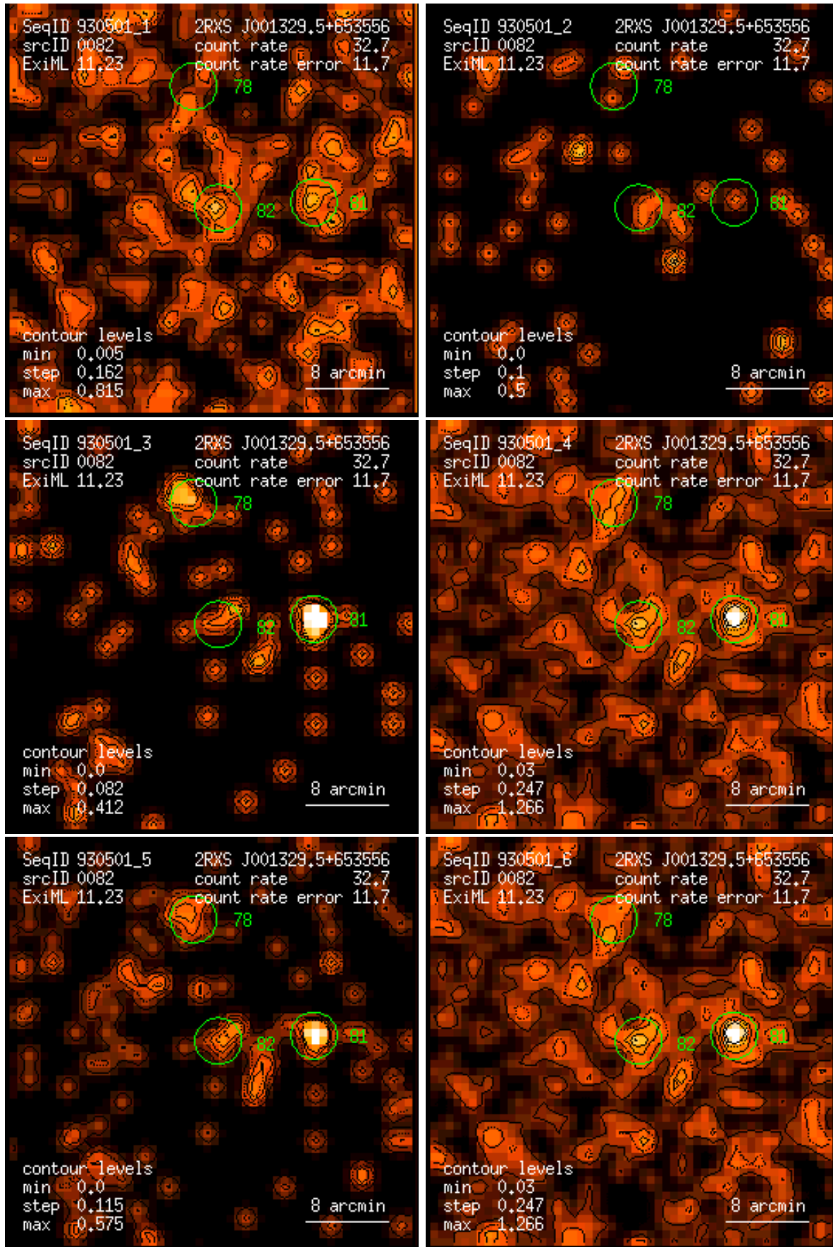
Figure 82: RASS 930501: detection 0082: band rate images, Gaussian filter: (1) PSPC channels 11 – 41, (2) 52 – 90, (3) 91 – 201, (4) 11 – 235, (5) 52 – 201, (6) 11 – 201. Broad band rates in counts/ks. Band rate contour levels in counts/ks/arcmin 2 .
