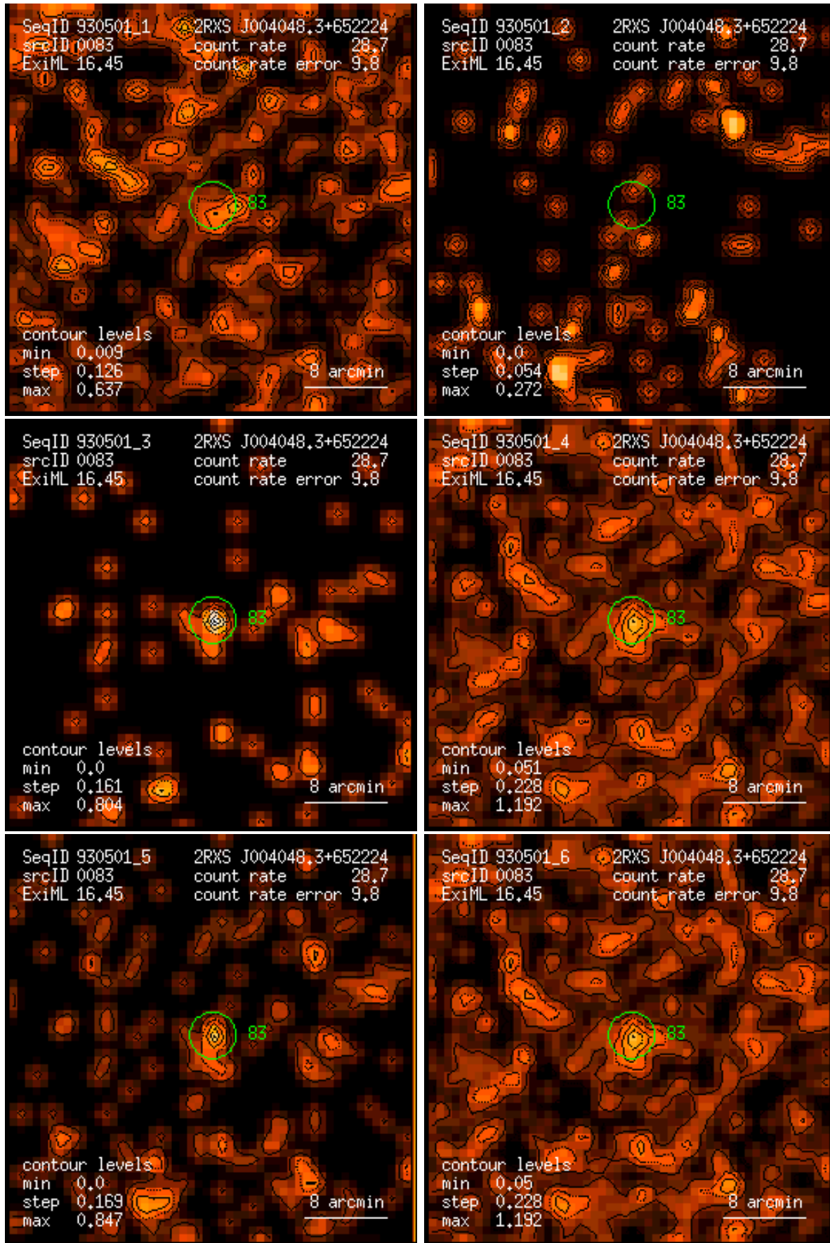
Figure 83: RASS 930501: detection 0083: band rate images, Gaussian filter: (1) PSPC channels 11 – 41, (2) 52 – 90, (3) 91 – 201, (4) 11 – 235, (5) 52 – 201, (6) 11 – 201. Broad band rates in counts/ks. Band rate contour levels in counts/ks/arcmin 2 .
