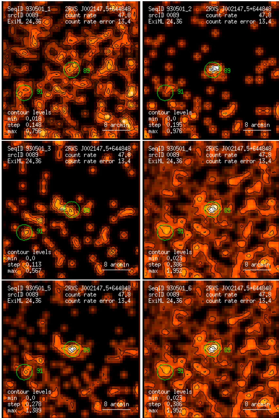
Figure 89: RASS 930501: detection 0089: band rate images, Gaussian filter: (1) PSPC channels 11 – 41, (2) 52 – 90, (3) 91 – 201, (4) 11 – 235, (5) 52 – 201, (6) 11 – 201. Broad band rates in counts/ks. Band rate contour levels in counts/ks/arcmin 2 .
