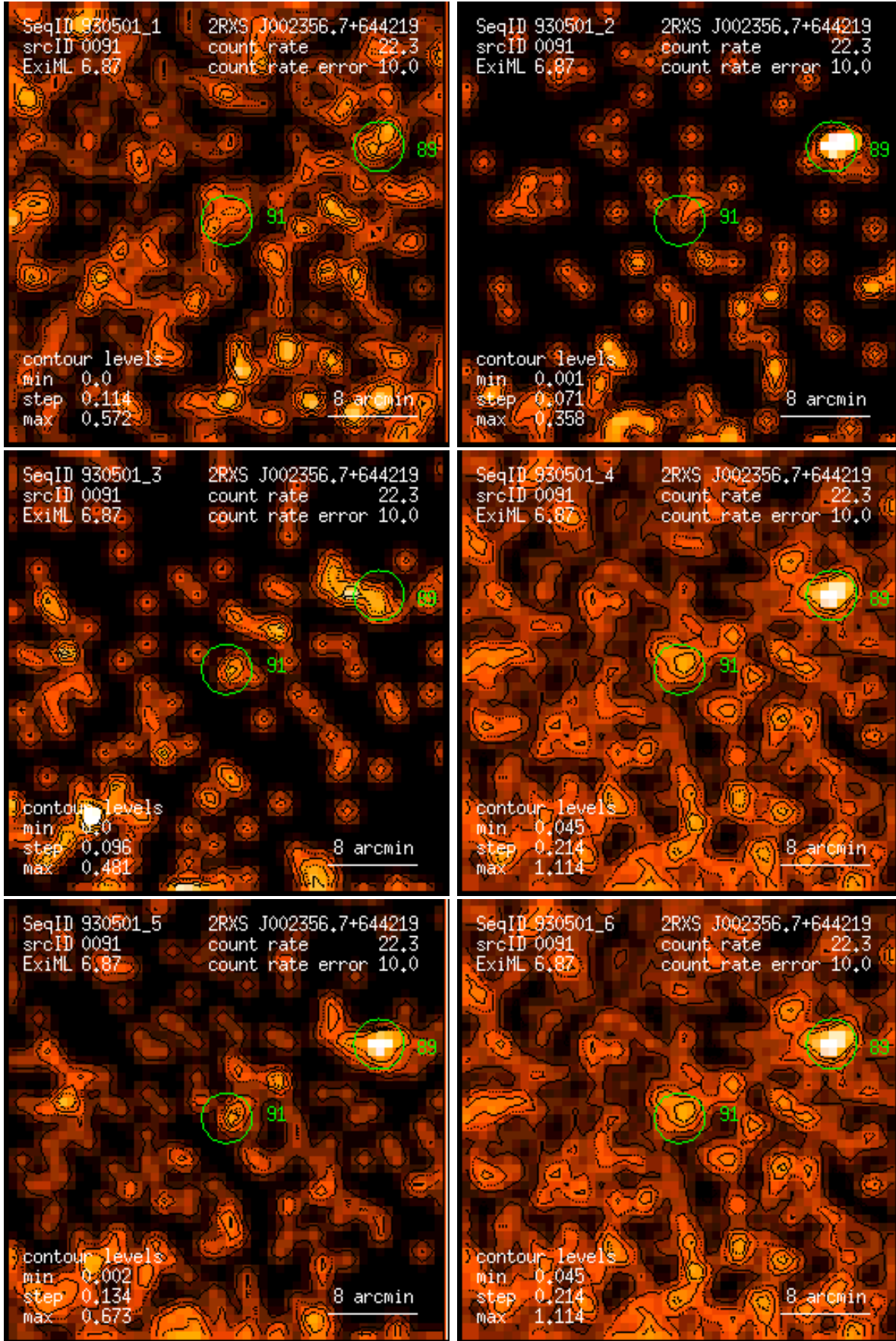
Figure 91: RASS 930501: detection 0091: band rate images, Gaussian filter: (1) PSPC channels 11 – 41, (2) 52 – 90, (3) 91 – 201, (4) 11 – 235, (5) 52 – 201, (6) 11 – 201. Broad band rates in counts/ks. Band rate contour levels in counts/ks/arcmin 2 .
