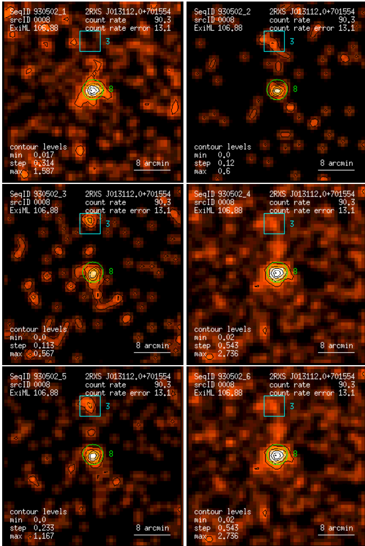
Figure 8: RASS 930502: detection 0008: band rate images, Gaussian filter: (1) PSPC channels 11 – 41, (2) 52 – 90, (3) 91 – 201, (4) 11 – 235, (5) 52 – 201, (6) 11 – 201. Broad band rates in counts/ks. Band rate contour levels in counts/ks/arcmin 2 .
