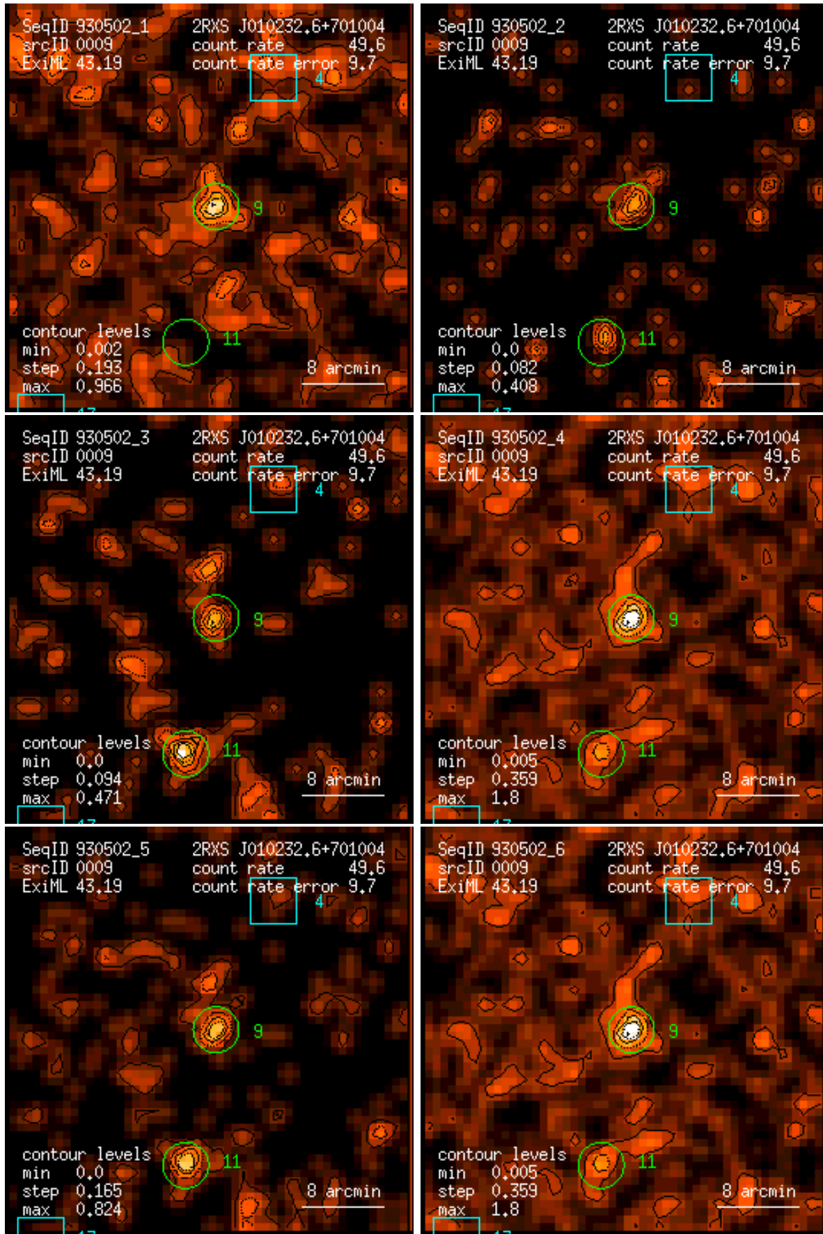
Figure 9: RASS 930502: detection 0009: band rate images, Gaussian filter: (1) PSPC channels 11 – 41, (2) 52 – 90, (3) 91 – 201, (4) 11 – 235, (5) 52 – 201, (6) 11 – 201. Broad band rates in counts/ks. Band rate contour levels in counts/ks/arcmin 2 .
