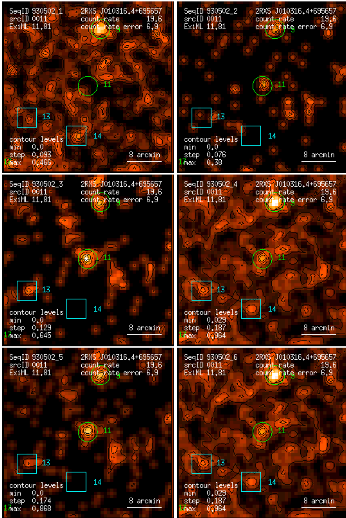
Figure 11: RASS 930502: detection 0011: band rate images, Gaussian filter: (1) PSPC channels 11 – 41, (2) 52 – 90, (3) 91 – 201, (4) 11 – 235, (5) 52 – 201, (6) 11 – 201. Broad band rates in counts/ks. Band rate contour levels in counts/ks/arcmin 2 .
