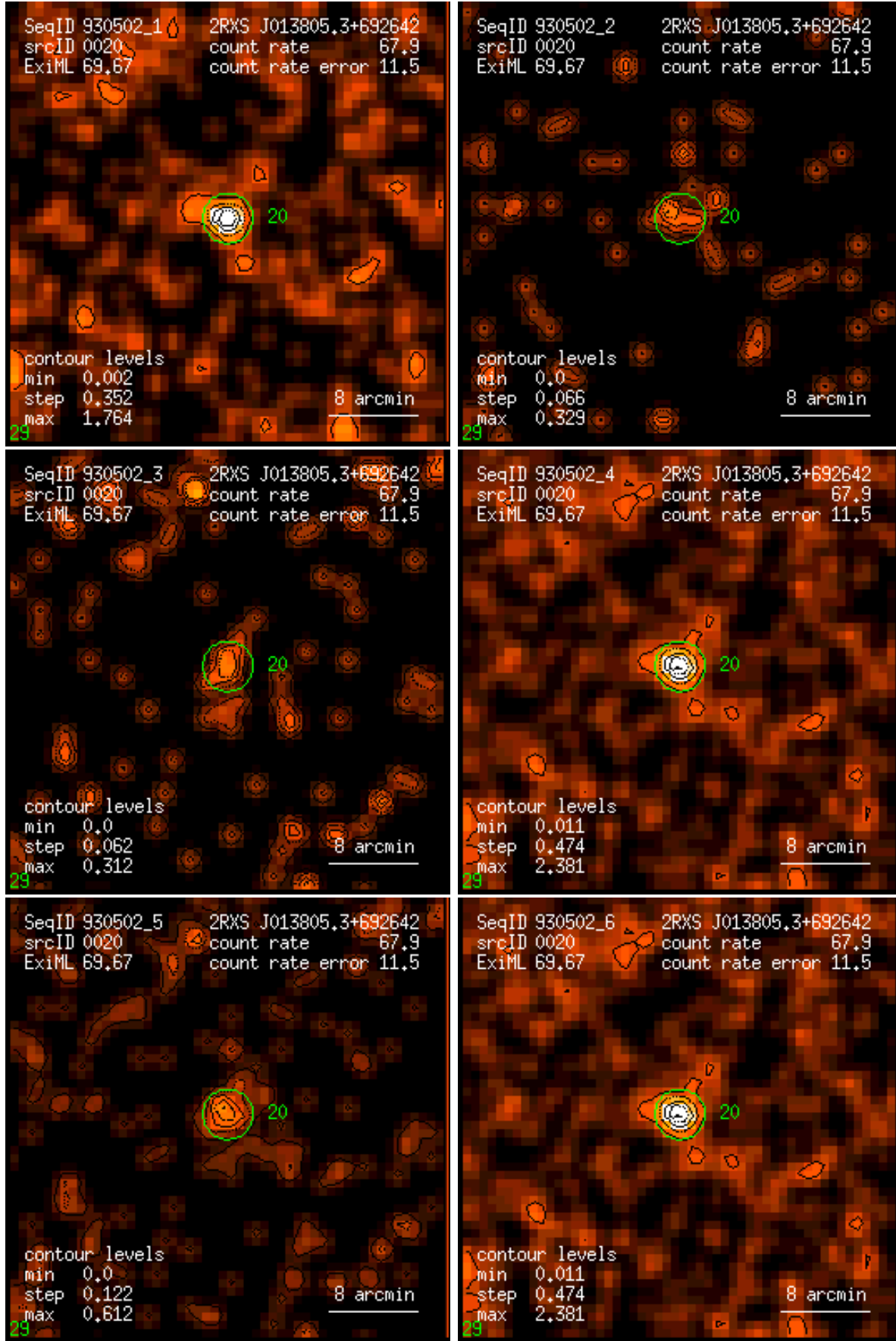
Figure 20: RASS 930502: detection 0020: band rate images, Gaussian filter: (1) PSPC channels 11 – 41, (2) 52 – 90, (3) 91 – 201, (4) 11 – 235, (5) 52 – 201, (6) 11 – 201. Broad band rates in counts/ks. Band rate contour levels in counts/ks/arcmin 2 .
