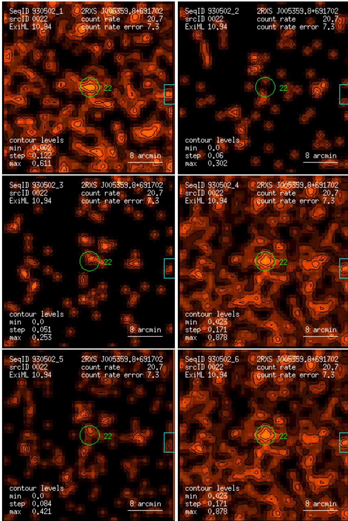
Figure 22: RASS 930502: detection 0022: band rate images, Gaussian filter: (1) PSPC channels 11 – 41, (2) 52 – 90, (3) 91 – 201, (4) 11 – 235, (5) 52 – 201, (6) 11 – 201. Broad band rates in counts/ks. Band rate contour levels in counts/ks/arcmin 2 .
