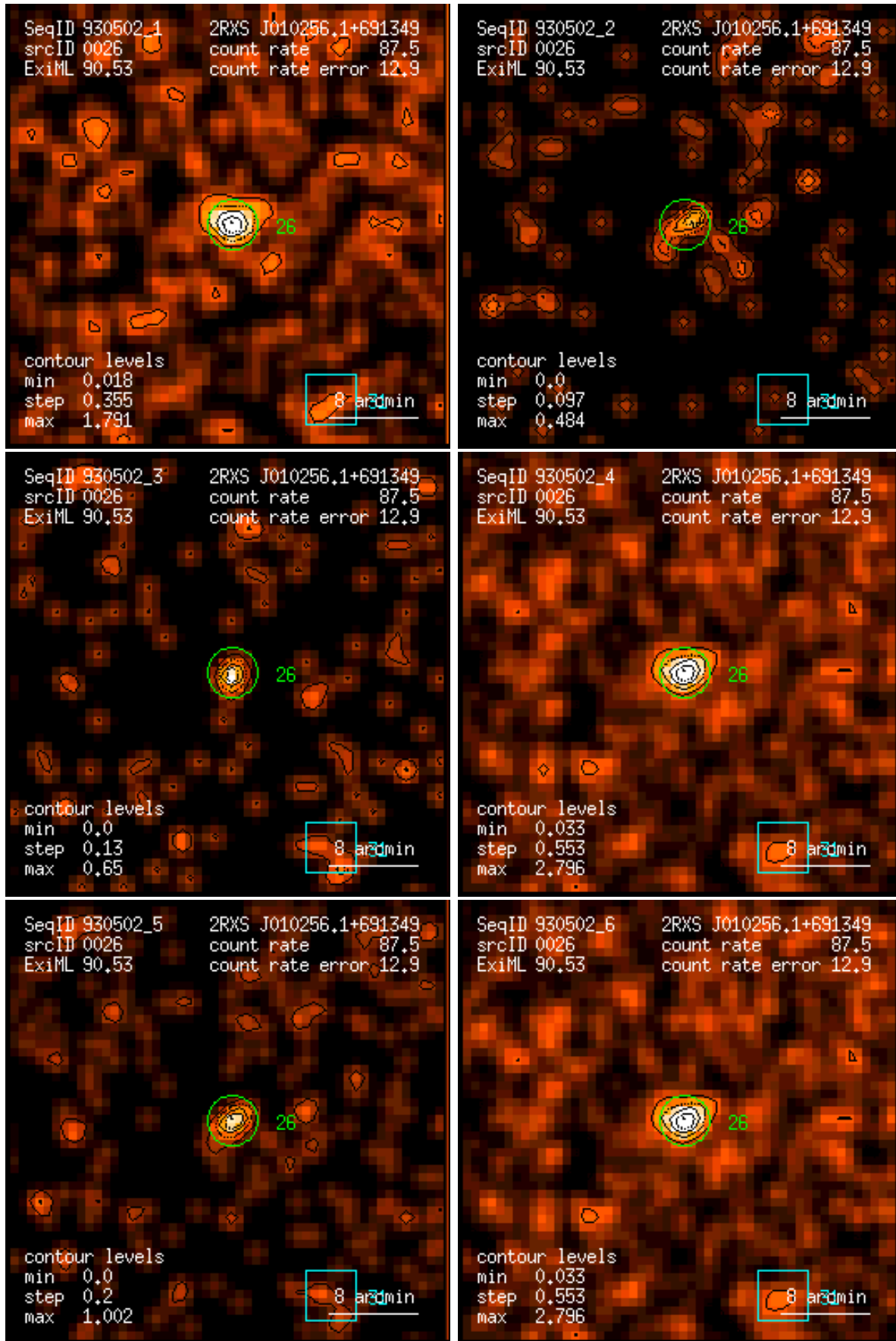
Figure 26: RASS 930502: detection 0026: band rate images, Gaussian filter: (1) PSPC channels 11 – 41, (2) 52 – 90, (3) 91 – 201, (4) 11 – 235, (5) 52 – 201, (6) 11 – 201. Broad band rates in counts/ks. Band rate contour levels in counts/ks/arcmin 2 .
