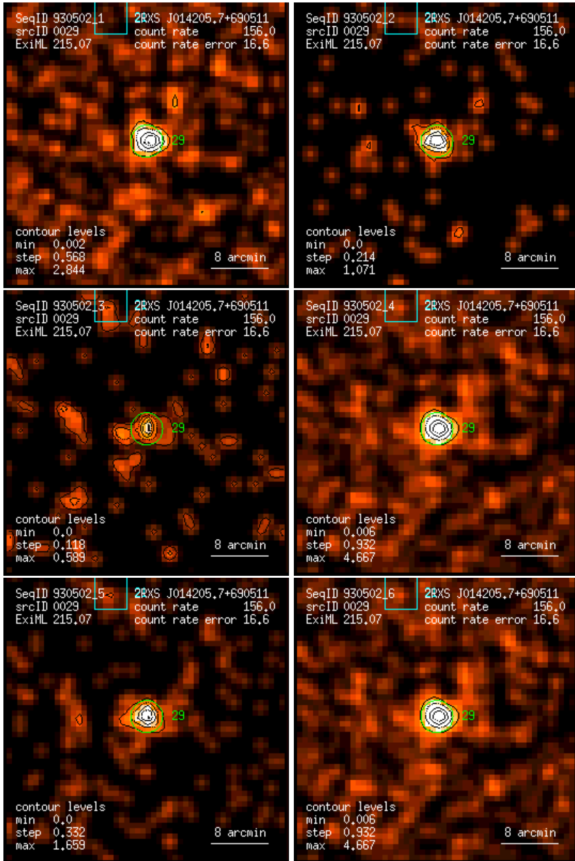
Figure 29: RASS 930502: detection 0029: band rate images, Gaussian filter: (1) PSPC channels 11 – 41, (2) 52 – 90, (3) 91 – 201, (4) 11 – 235, (5) 52 – 201, (6) 11 – 201. Broad band rates in counts/ks. Band rate contour levels in counts/ks/arcmin 2 .
