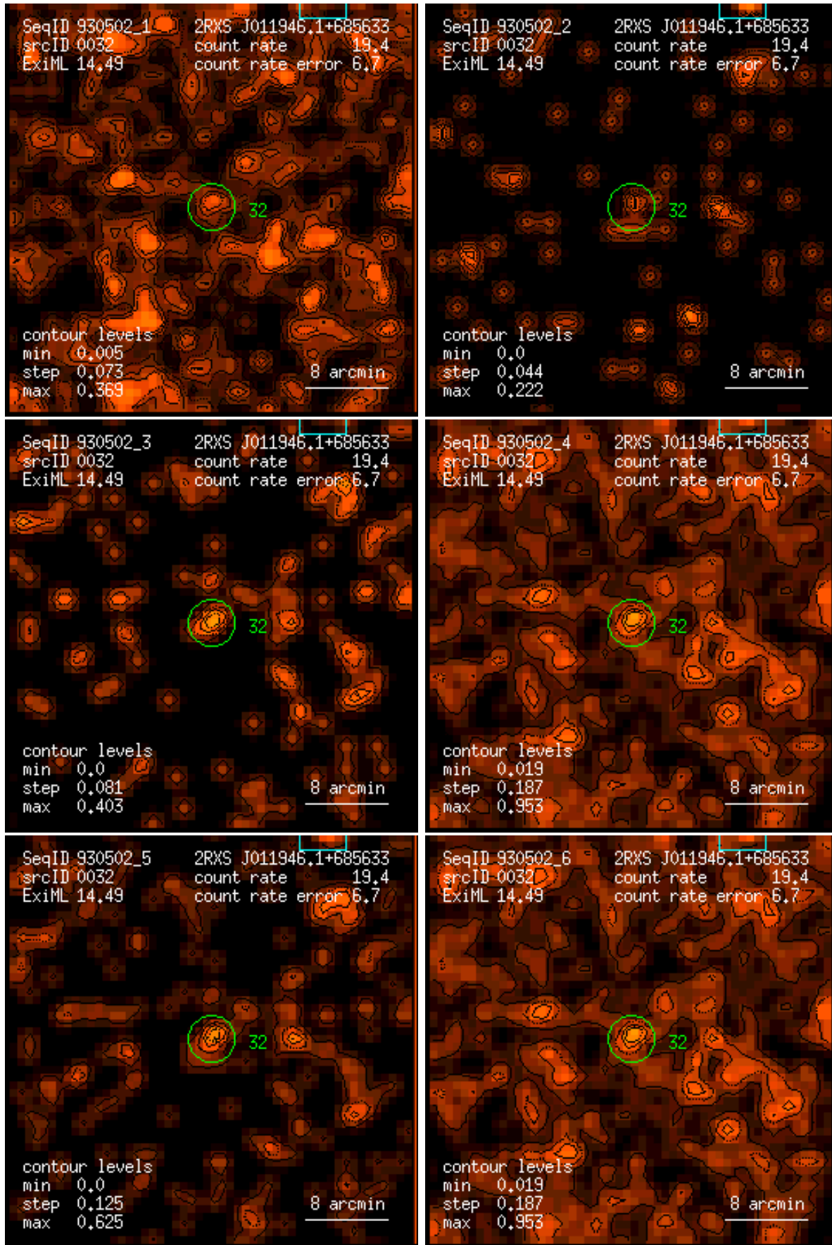
Figure 32: RASS 930502: detection 0032: band rate images, Gaussian filter: (1) PSPC channels 11 – 41, (2) 52 – 90, (3) 91 – 201, (4) 11 – 235, (5) 52 – 201, (6) 11 – 201. Broad band rates in counts/ks. Band rate contour levels in counts/ks/arcmin 2 .
