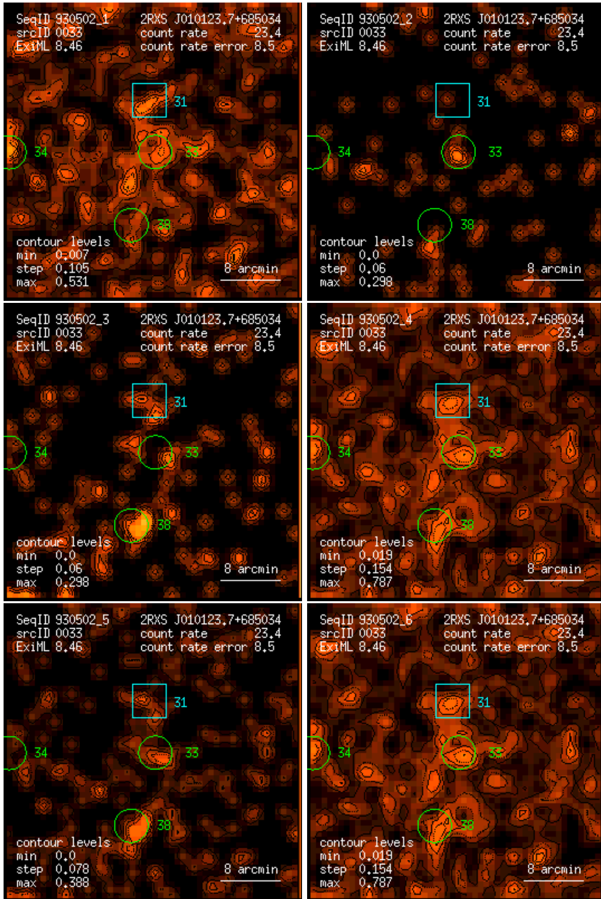
Figure 33: RASS 930502: detection 0033: band rate images, Gaussian filter: (1) PSPC channels 11 – 41, (2) 52 – 90, (3) 91 – 201, (4) 11 – 235, (5) 52 – 201, (6) 11 – 201. Broad band rates in counts/ks. Band rate contour levels in counts/ks/arcmin 2 .
