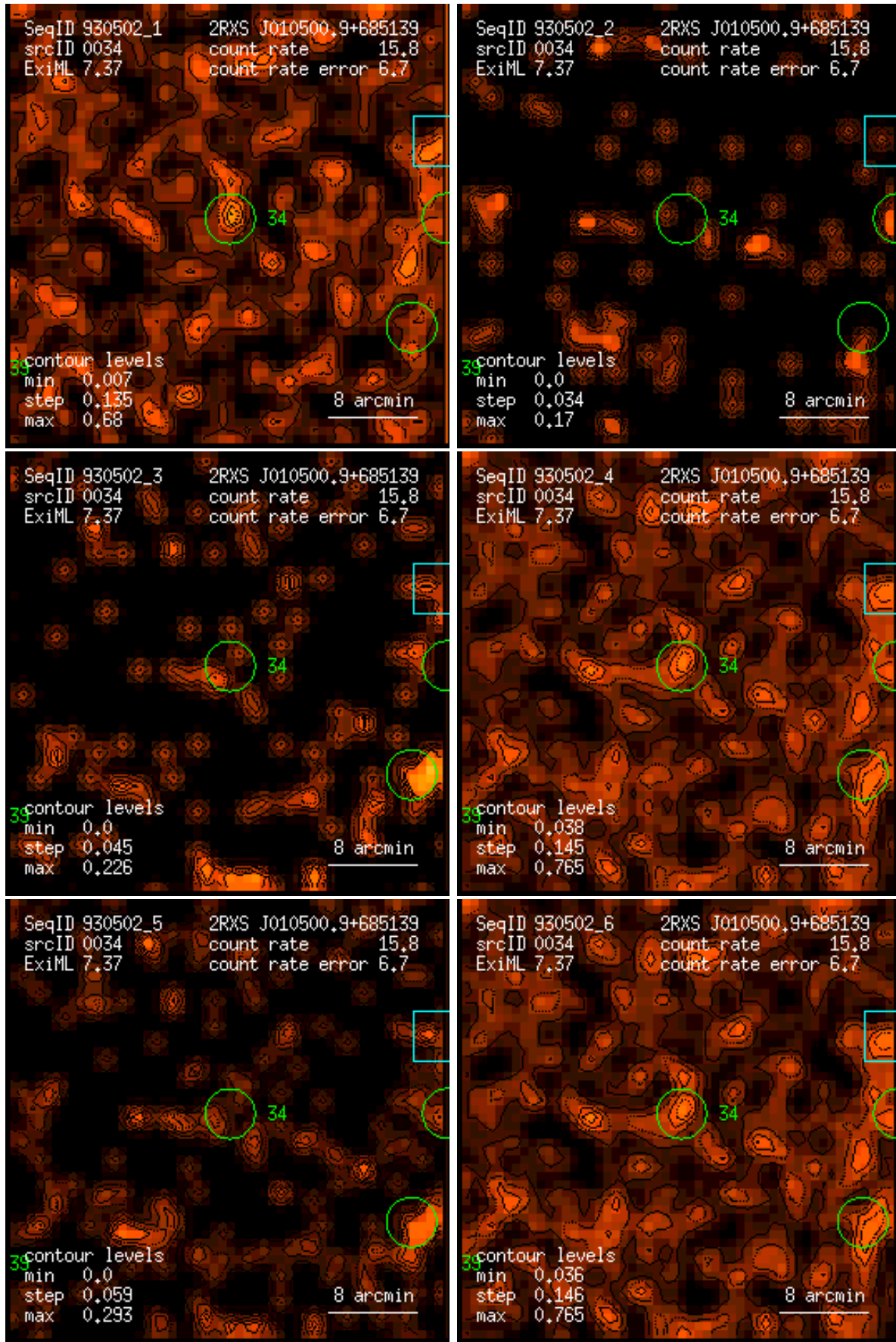
Figure 34: RASS 930502: detection 0034: band rate images, Gaussian filter: (1) PSPC channels 11 – 41, (2) 52 – 90, (3) 91 – 201, (4) 11 – 235, (5) 52 – 201, (6) 11 – 201. Broad band rates in counts/ks. Band rate contour levels in counts/ks/arcmin 2 .
