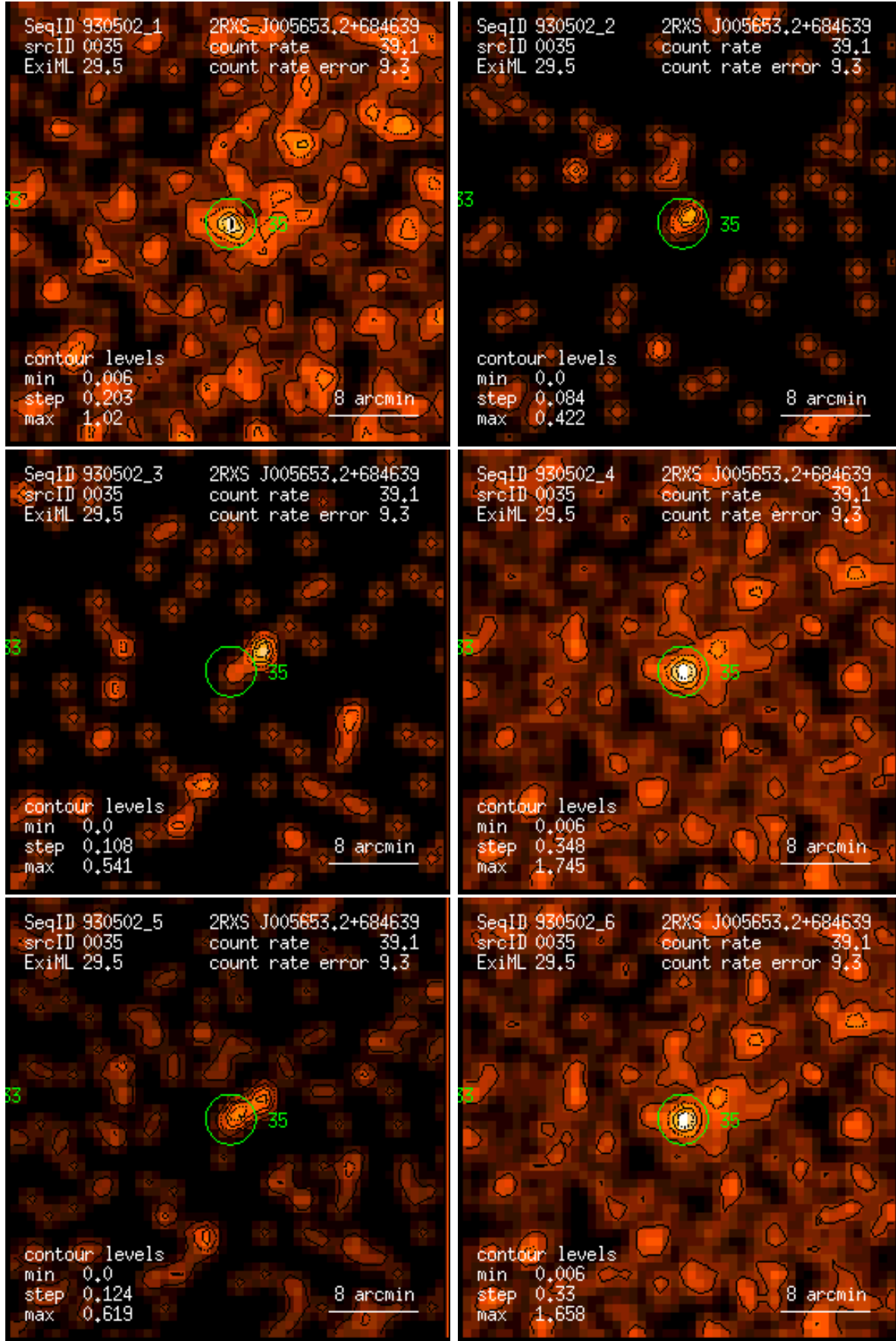
Figure 35: RASS 930502: detection 0035: band rate images, Gaussian filter: (1) PSPC channels 11 – 41, (2) 52 – 90, (3) 91 – 201, (4) 11 – 235, (5) 52 – 201, (6) 11 – 201. Broad band rates in counts/ks. Band rate contour levels in counts/ks/arcmin 2 .
