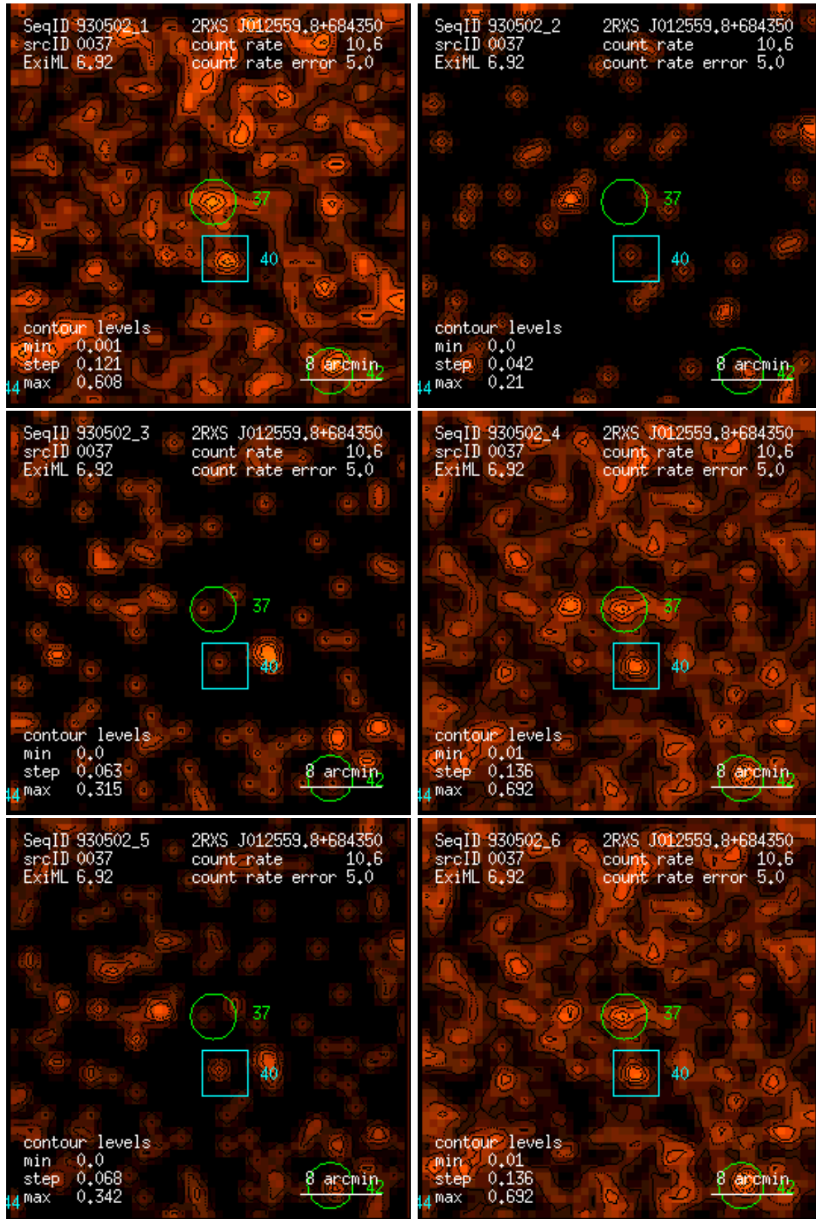
Figure 37: RASS 930502: detection 0037: band rate images, Gaussian filter: (1) PSPC channels 11 – 41, (2) 52 – 90, (3) 91 – 201, (4) 11 – 235, (5) 52 – 201, (6) 11 – 201. Broad band rates in counts/ks. Band rate contour levels in counts/ks/arcmin 2 .
