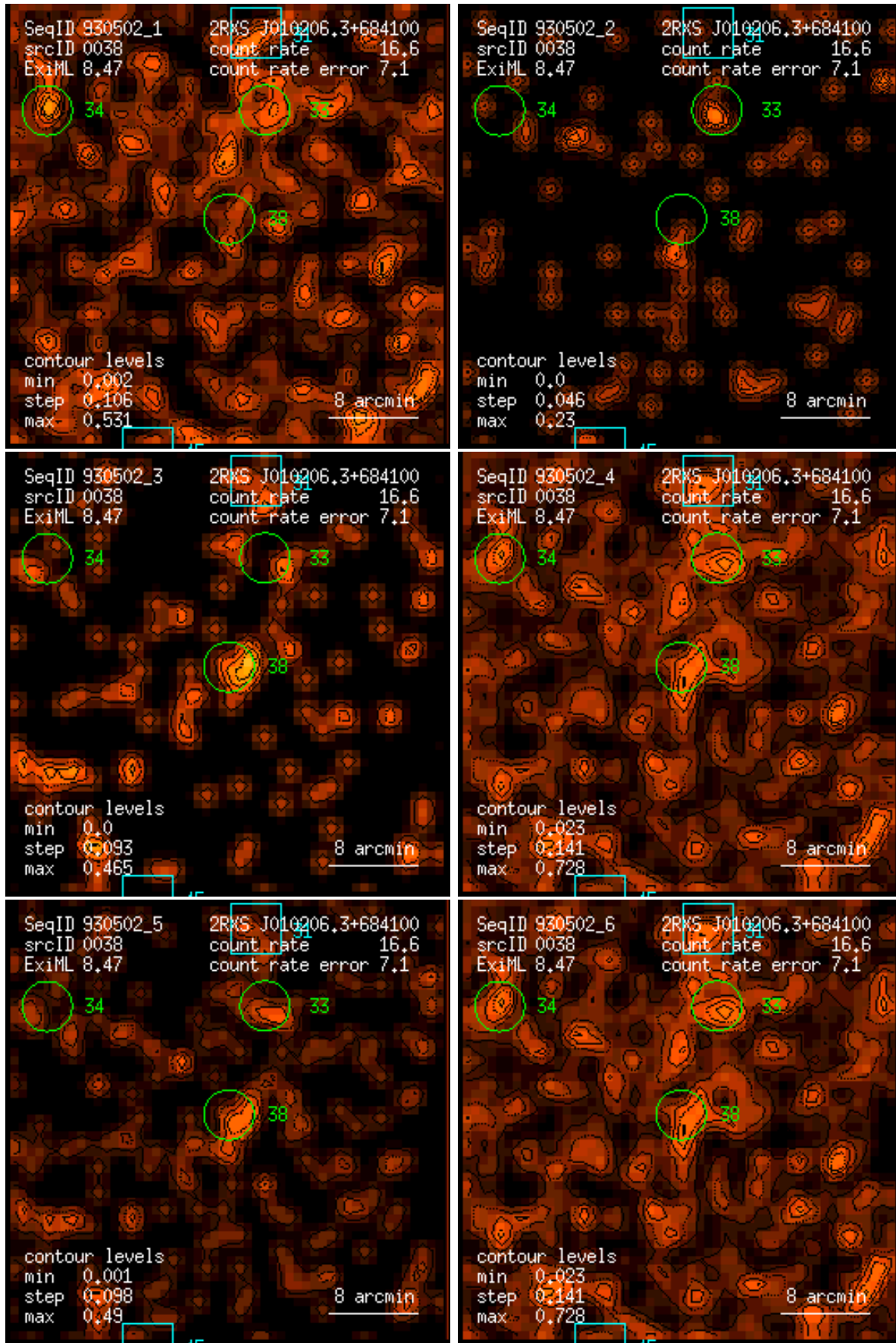
Figure 38: RASS 930502: detection 0038: band rate images, Gaussian filter: (1) PSPC channels 11 – 41, (2) 52 – 90, (3) 91 – 201, (4) 11 – 235, (5) 52 – 201, (6) 11 – 201. Broad band rates in counts/ks. Band rate contour levels in counts/ks/arcmin 2 .
