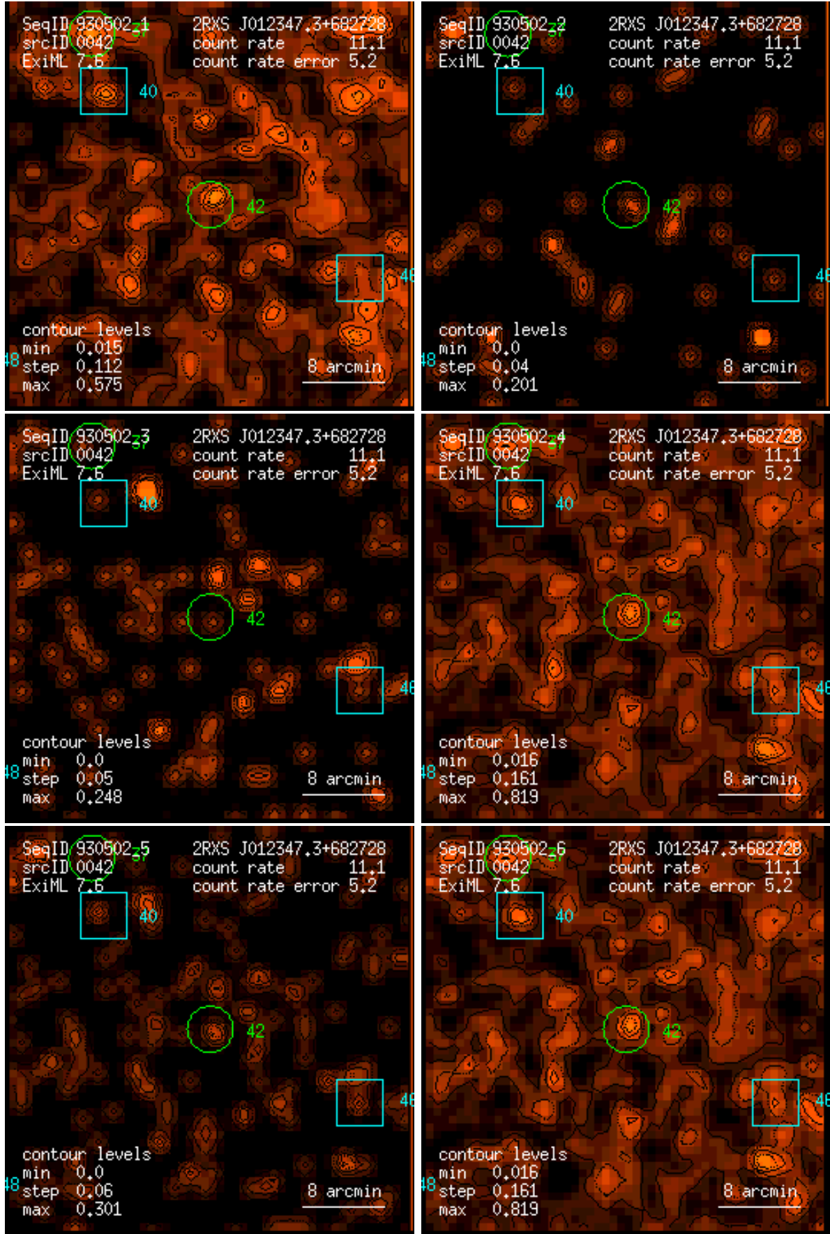
Figure 42: RASS 930502: detection 0042: band rate images, Gaussian filter: (1) PSPC channels 11 – 41, (2) 52 – 90, (3) 91 – 201, (4) 11 – 235, (5) 52 – 201, (6) 11 – 201. Broad band rates in counts/ks. Band rate contour levels in counts/ks/arcmin 2 .
