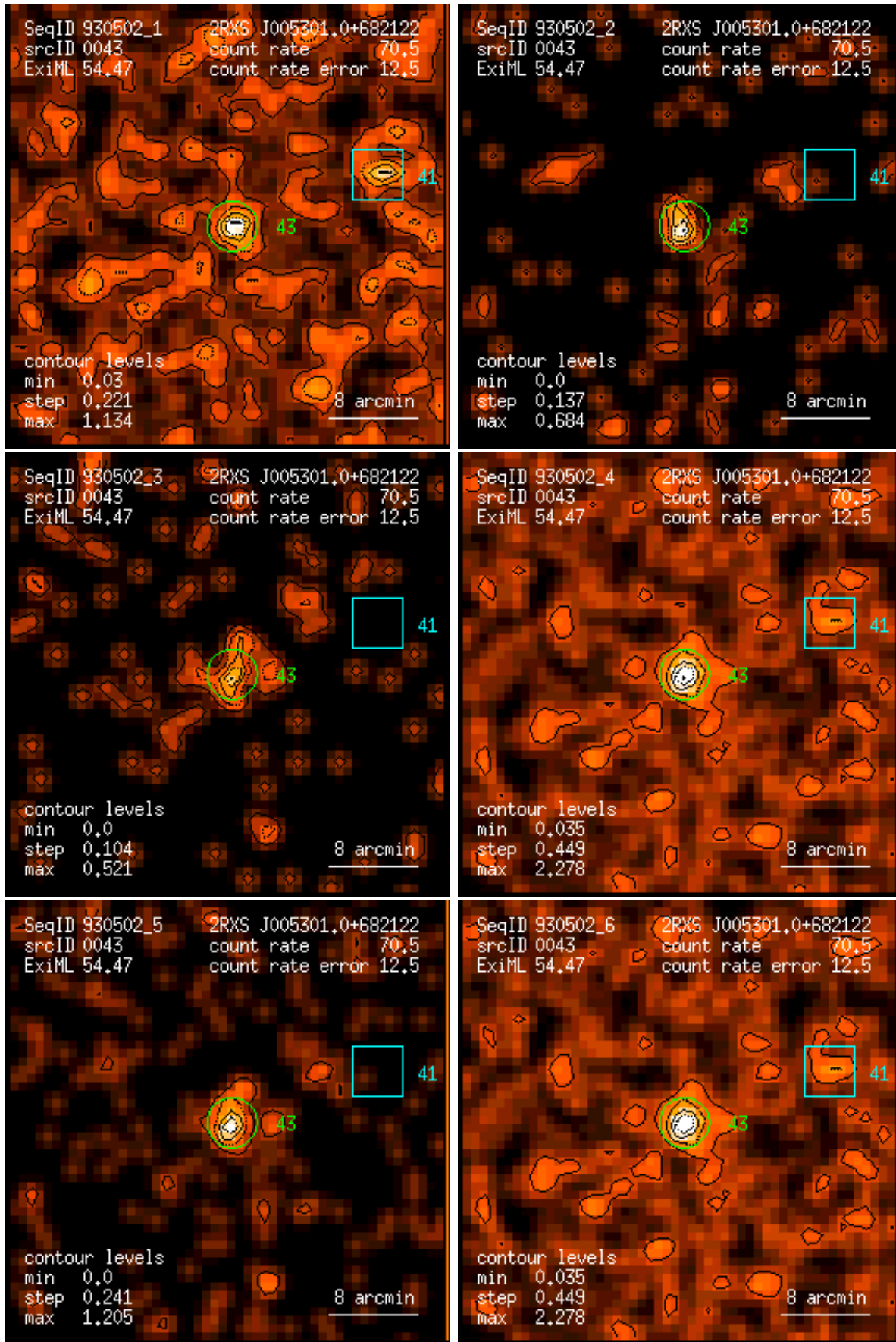
Figure 43: RASS 930502: detection 0043: band rate images, Gaussian filter: (1) PSPC channels 11 – 41, (2) 52 – 90, (3) 91 – 201, (4) 11 – 235, (5) 52 – 201, (6) 11 – 201. Broad band rates in counts/ks. Band rate contour levels in counts/ks/arcmin 2 .
