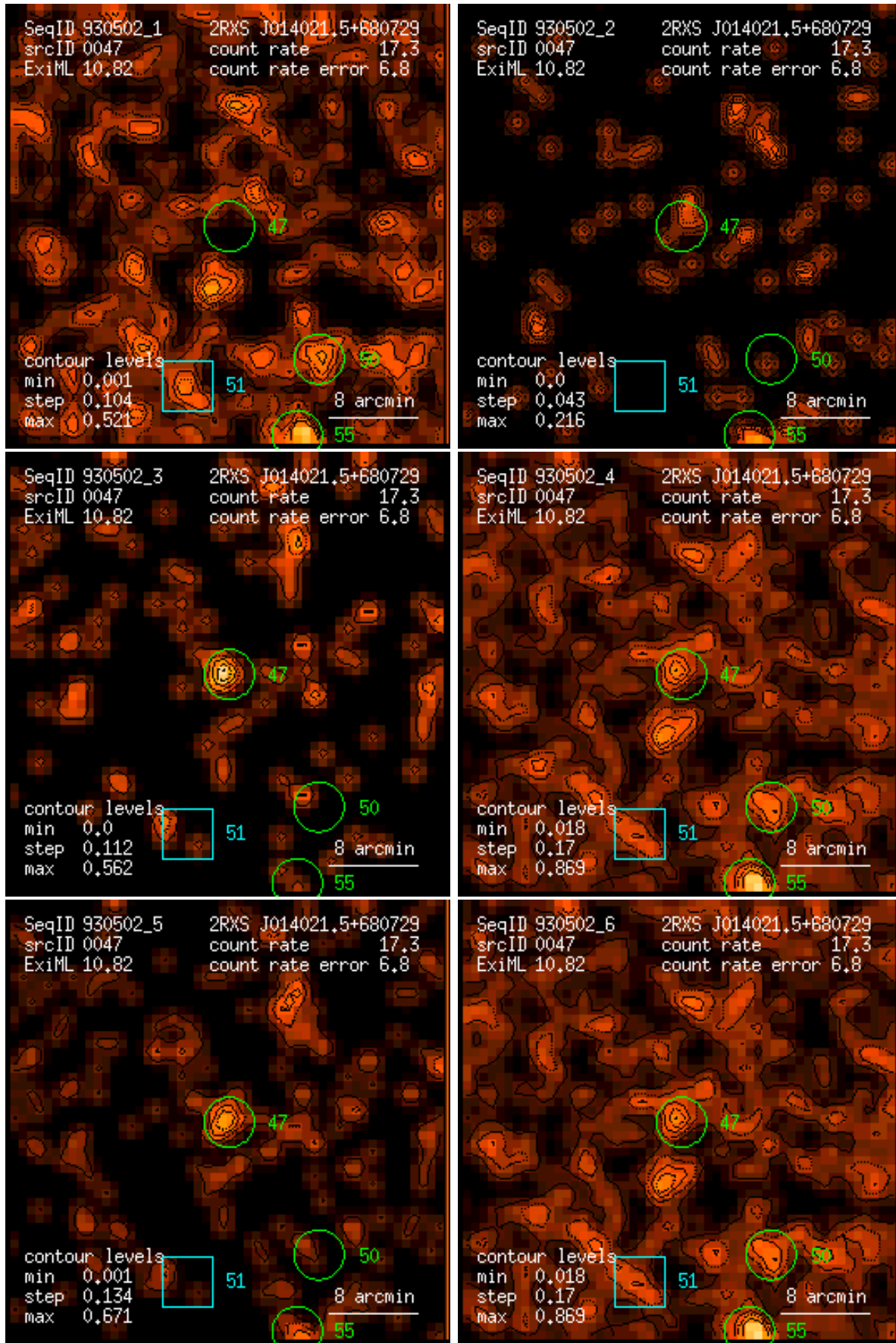
Figure 47: RASS 930502: detection 0047: band rate images, Gaussian filter: (1) PSPC channels 11 – 41, (2) 52 – 90, (3) 91 – 201, (4) 11 – 235, (5) 52 – 201, (6) 11 – 201. Broad band rates in counts/ks. Band rate contour levels in counts/ks/arcmin 2 .
