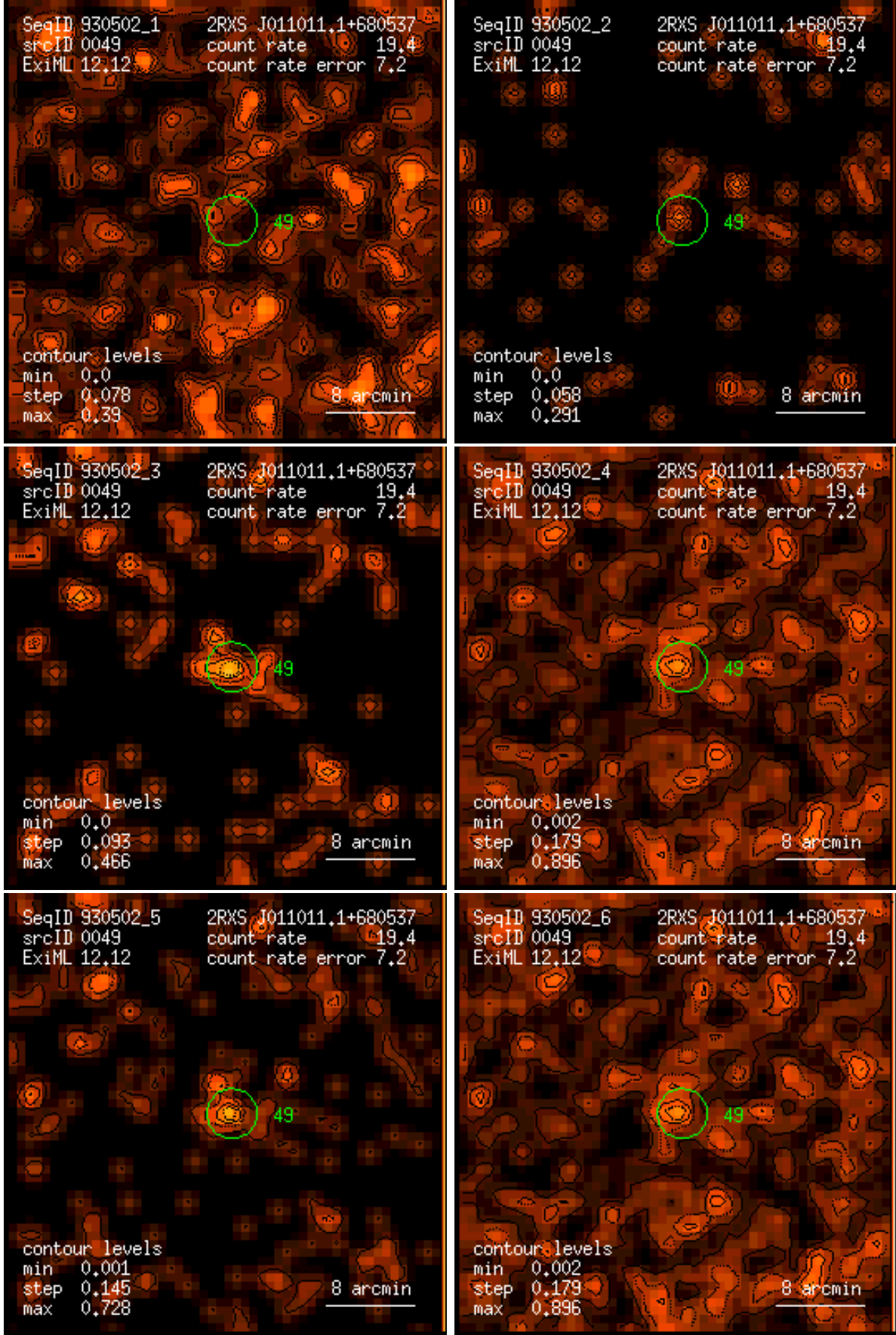
Figure 49: RASS 930502: detection 0049: band rate images, Gaussian filter: (1) PSPC channels 11 – 41, (2) 52 – 90, (3) 91 – 201, (4) 11 – 235, (5) 52 – 201, (6) 11 – 201. Broad band rates in counts/ks. Band rate contour levels in counts/ks/arcmin 2 .
