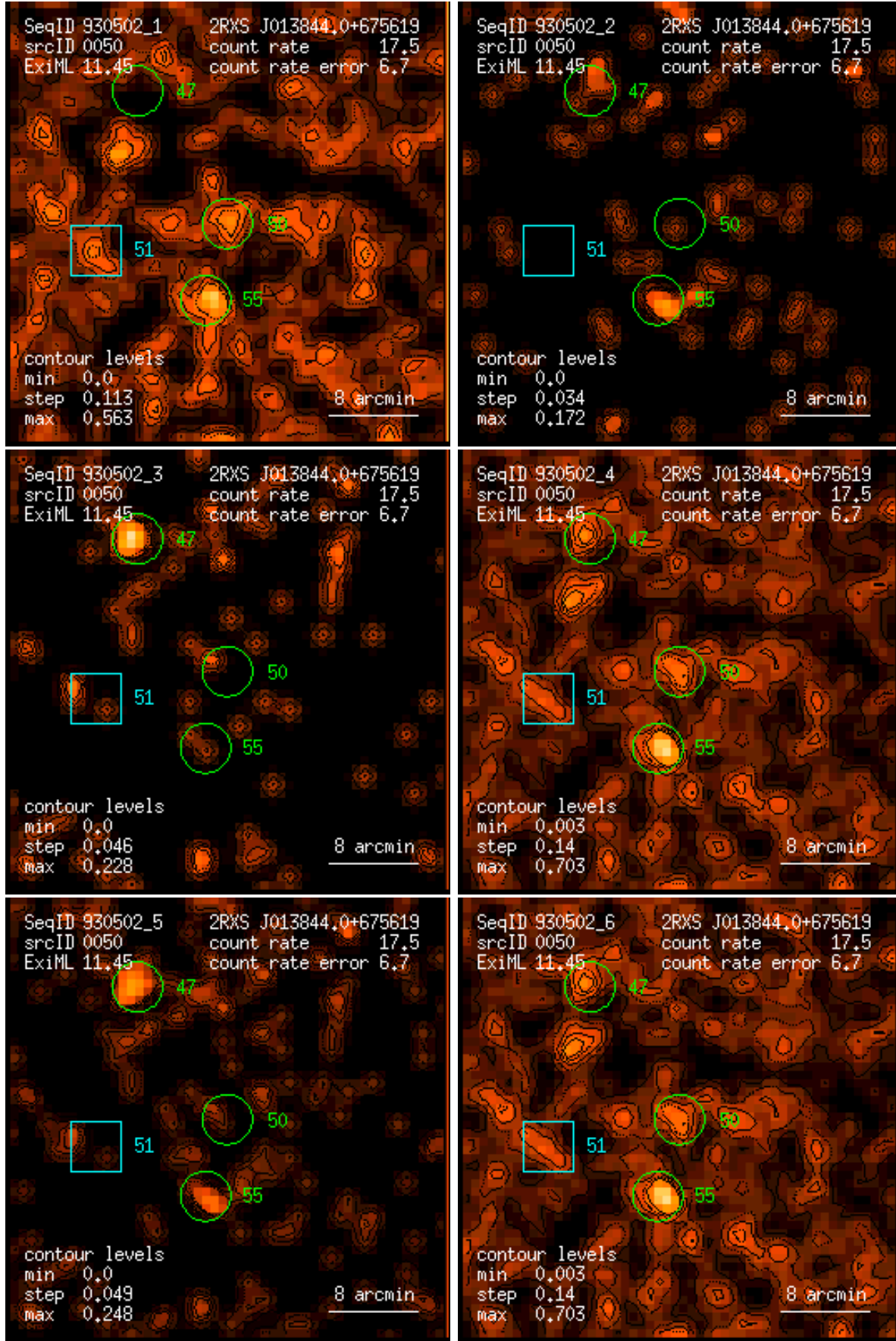
Figure 50: RASS 930502: detection 0050: band rate images, Gaussian filter: (1) PSPC channels 11 – 41, (2) 52 – 90, (3) 91 – 201, (4) 11 – 235, (5) 52 – 201, (6) 11 – 201. Broad band rates in counts/ks. Band rate contour levels in counts/ks/arcmin 2 .
