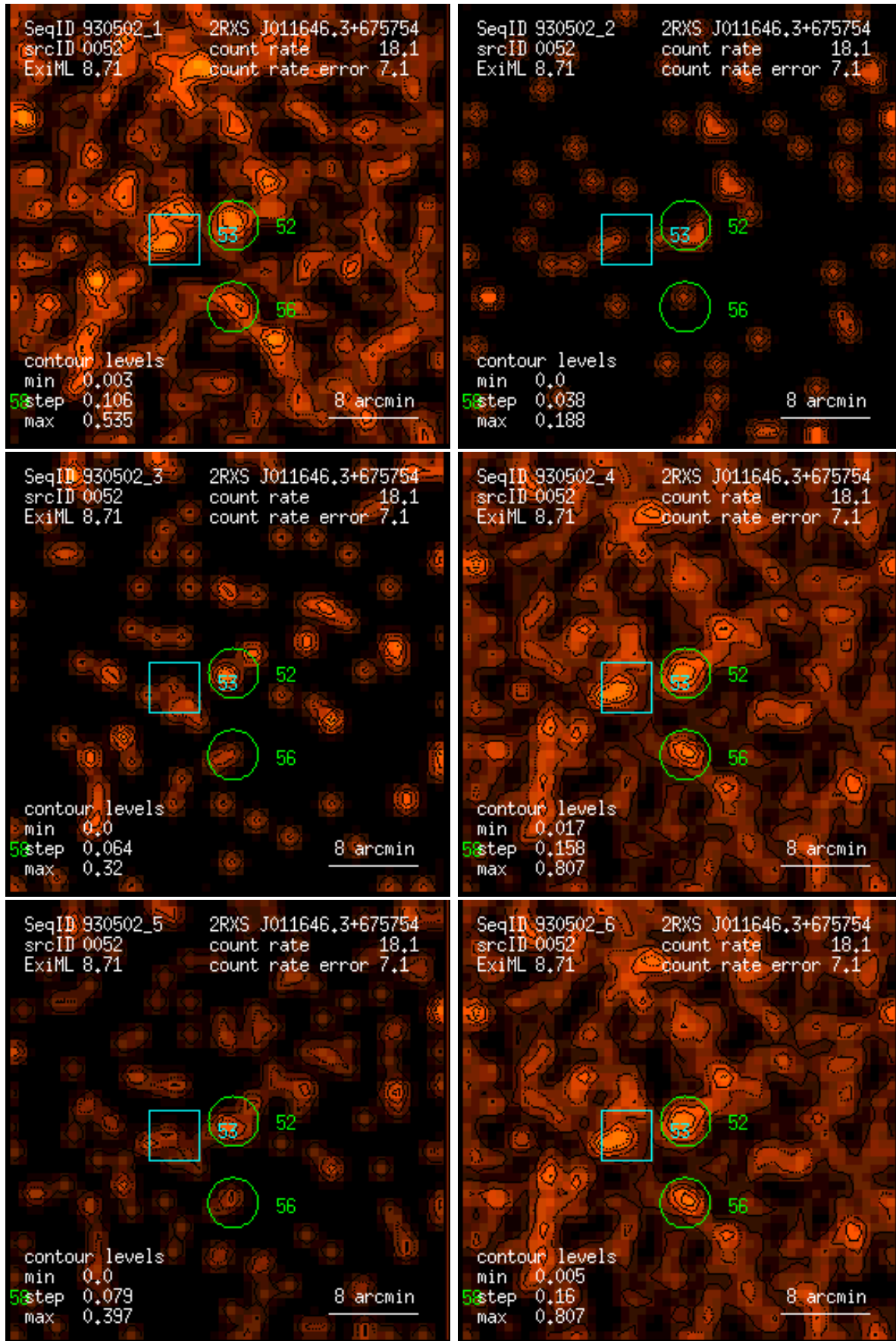
Figure 52: RASS 930502: detection 0052: band rate images, Gaussian filter: (1) PSPC channels 11 – 41, (2) 52 – 90, (3) 91 – 201, (4) 11 – 235, (5) 52 – 201, (6) 11 – 201. Broad band rates in counts/ks. Band rate contour levels in counts/ks/arcmin 2 .
