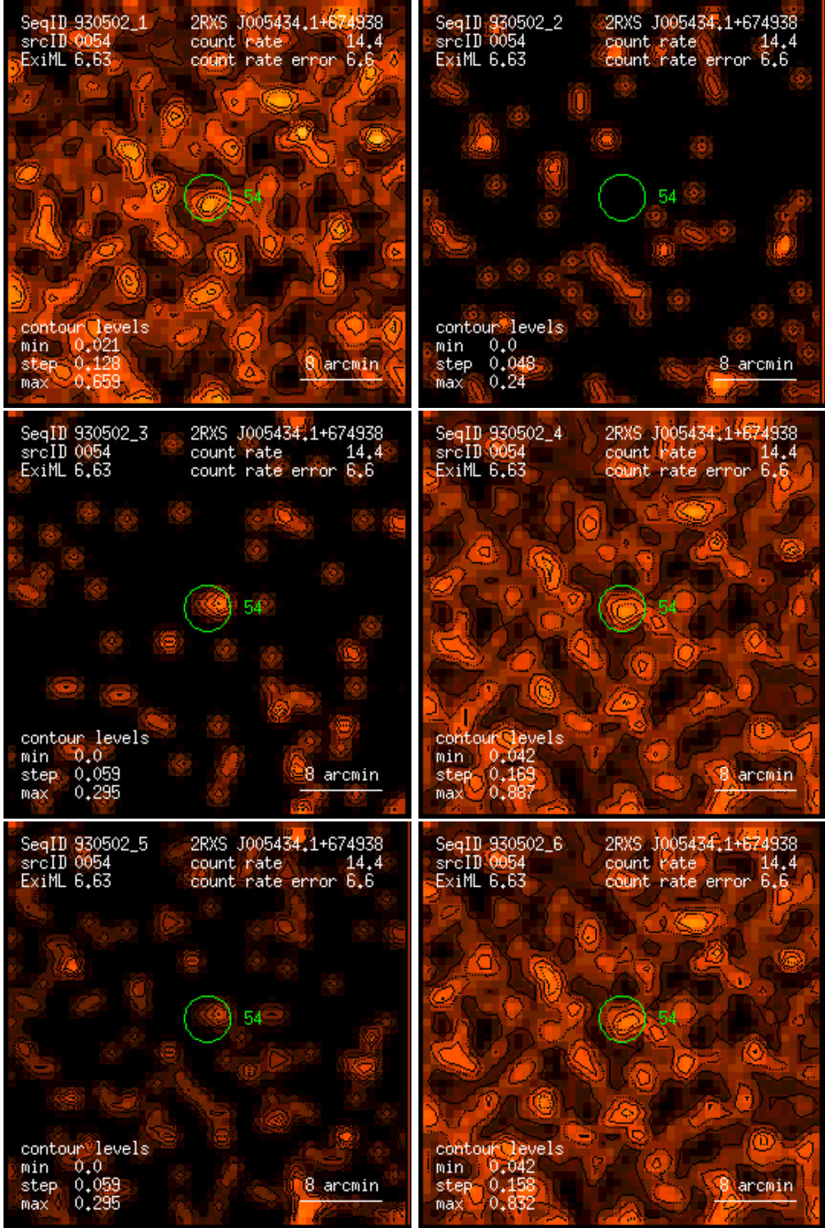
Figure 54: RASS 930502: detection 0054: band rate images, Gaussian filter: (1) PSPC channels 11 – 41, (2) 52 – 90, (3) 91 – 201, (4) 11 – 235, (5) 52 – 201, (6) 11 – 201. Broad band rates in counts/ks. Band rate contour levels in counts/ks/arcmin 2 .
