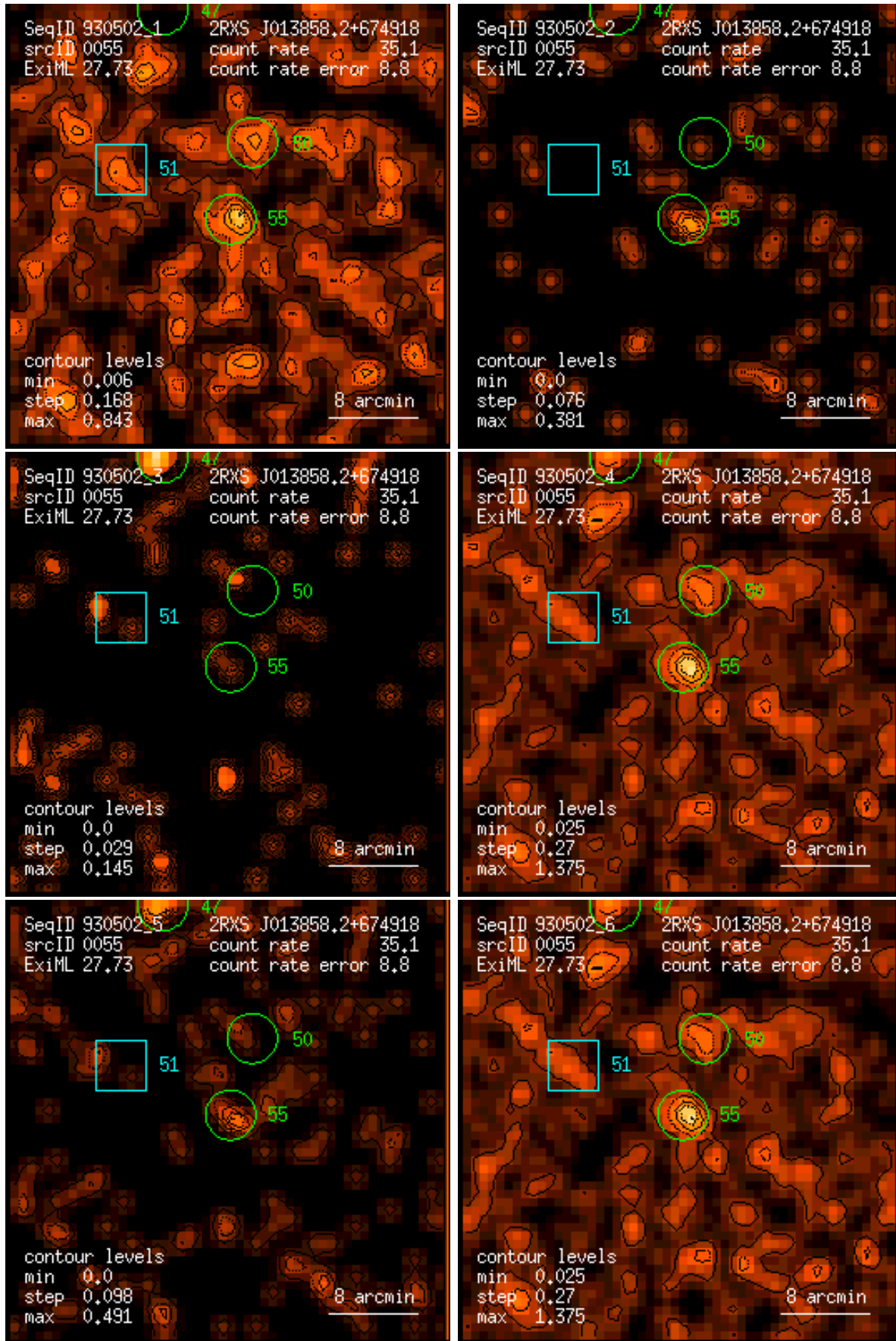
Figure 55: RASS 930502: detection 0055: band rate images, Gaussian filter: (1) PSPC channels 11 – 41, (2) 52 – 90, (3) 91 – 201, (4) 11 – 235, (5) 52 – 201, (6) 11 – 201. Broad band rates in counts/ks. Band rate contour levels in counts/ks/arcmin 2 .
