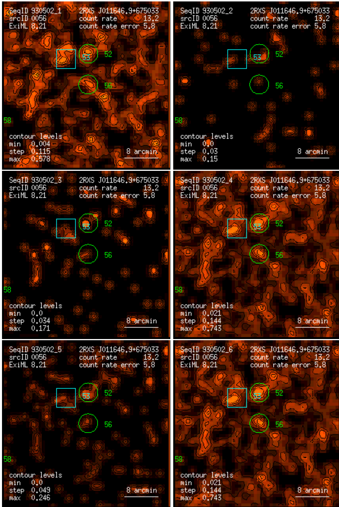
Figure 56: RASS 930502: detection 0056: band rate images, Gaussian filter: (1) PSPC channels 11 – 41, (2) 52 – 90, (3) 91 – 201, (4) 11 – 235, (5) 52 – 201, (6) 11 – 201. Broad band rates in counts/ks. Band rate contour levels in counts/ks/arcmin 2 .
