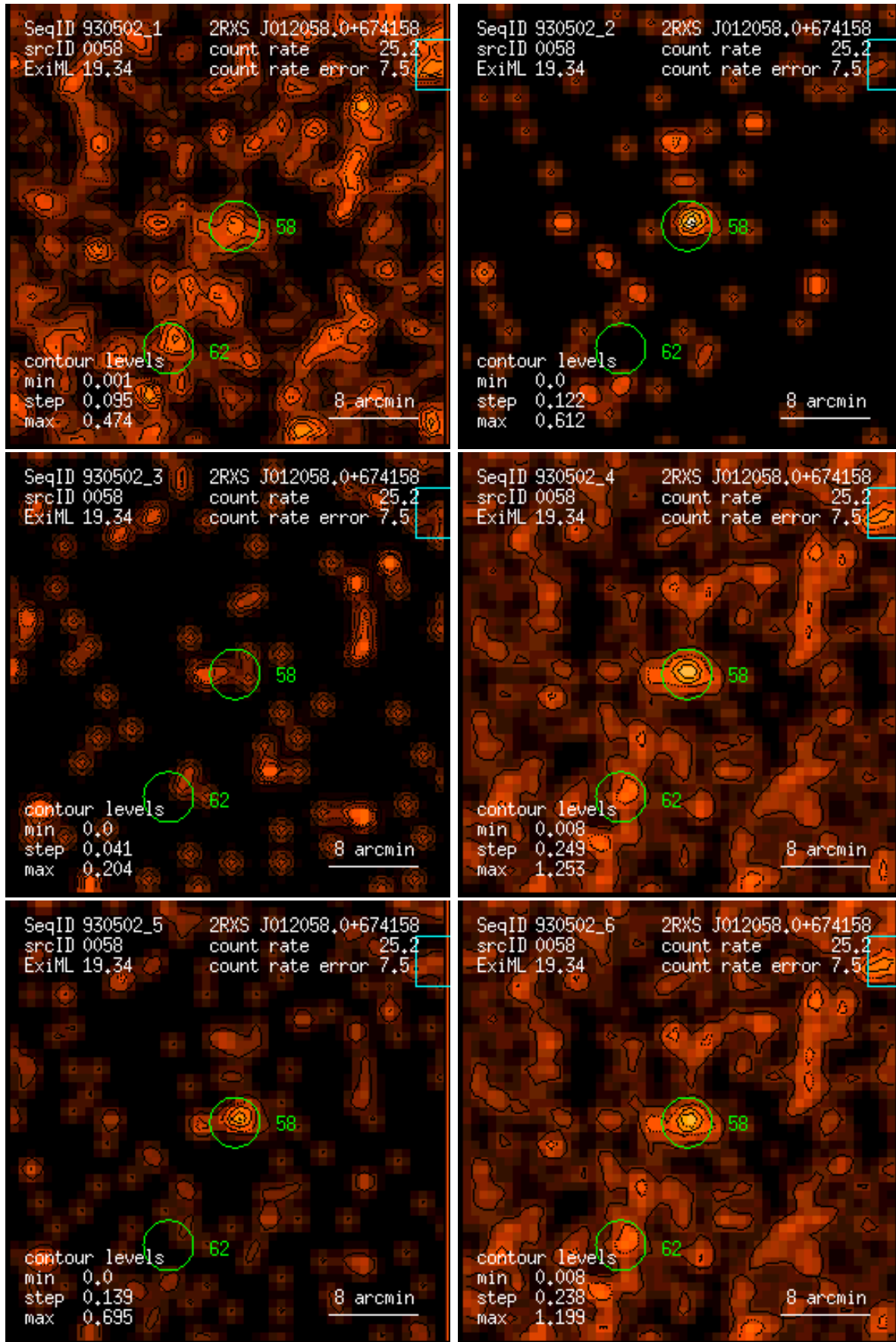
Figure 58: RASS 930502: detection 0058: band rate images, Gaussian filter: (1) PSPC channels 11 – 41, (2) 52 – 90, (3) 91 – 201, (4) 11 – 235, (5) 52 – 201, (6) 11 – 201. Broad band rates in counts/ks. Band rate contour levels in counts/ks/arcmin 2 .
