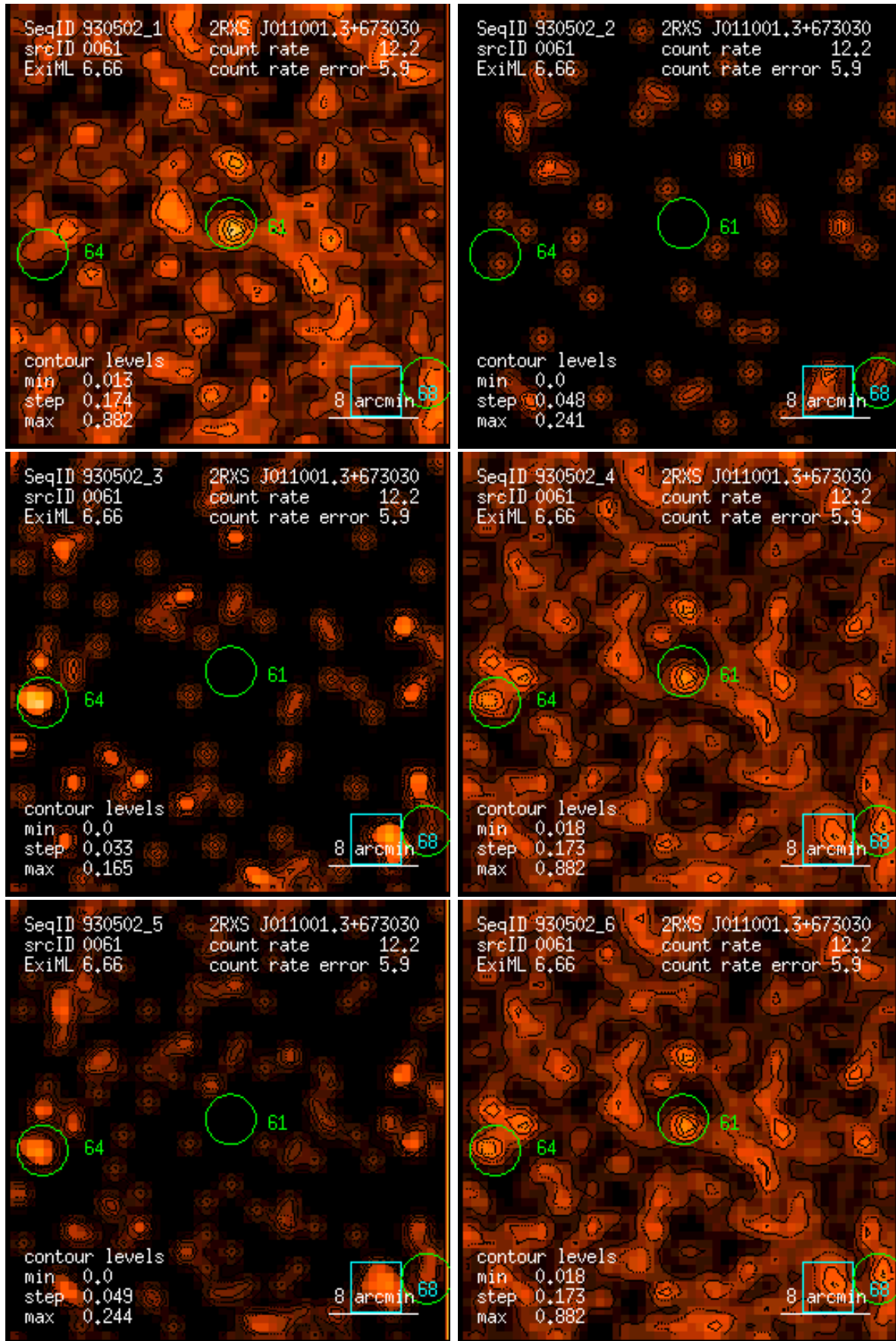
Figure 61: RASS 930502: detection 0061: band rate images, Gaussian filter: (1) PSPC channels 11 – 41, (2) 52 – 90, (3) 91 – 201, (4) 11 – 235, (5) 52 – 201, (6) 11 – 201. Broad band rates in counts/ks. Band rate contour levels in counts/ks/arcmin 2 .
