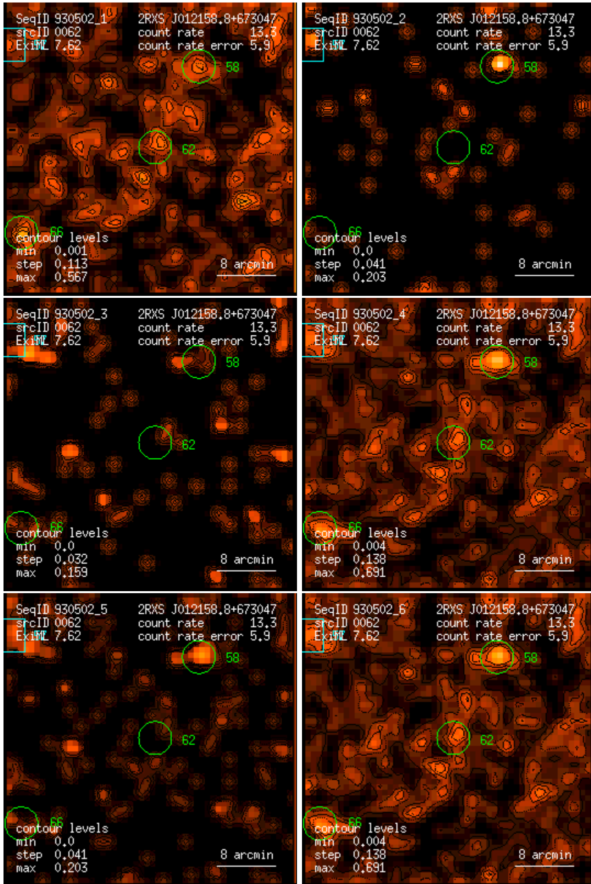
Figure 62: RASS 930502: detection 0062: band rate images, Gaussian filter: (1) PSPC channels 11 – 41, (2) 52 – 90, (3) 91 – 201, (4) 11 – 235, (5) 52 – 201, (6) 11 – 201. Broad band rates in counts/ks. Band rate contour levels in counts/ks/arcmin 2 .
