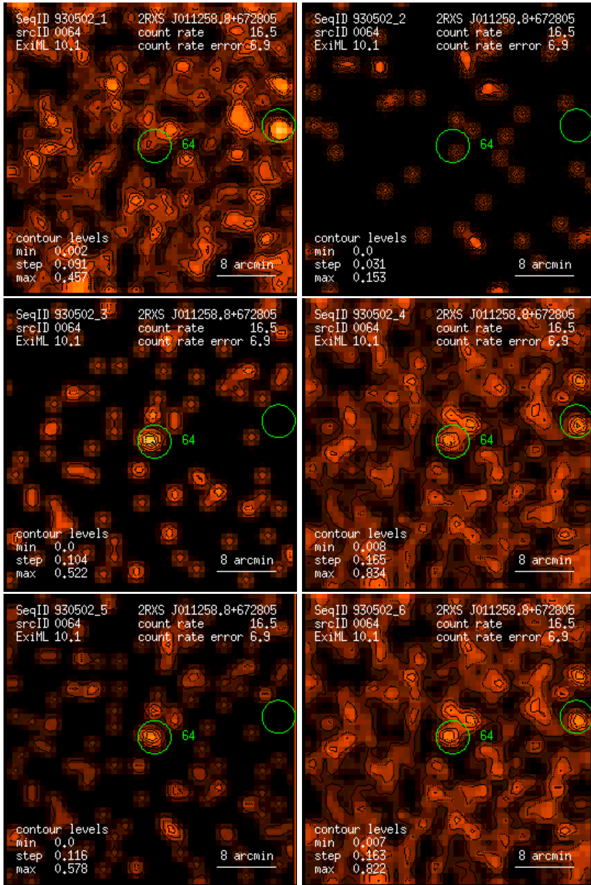
Figure 64: RASS 930502: detection 0064: band rate images, Gaussian filter: (1) PSPC channels 11 – 41, (2) 52 – 90, (3) 91 – 201, (4) 11 – 235, (5) 52 – 201, (6) 11 – 201. Broad band rates in counts/ks. Band rate contour levels in counts/ks/arcmin 2 .
