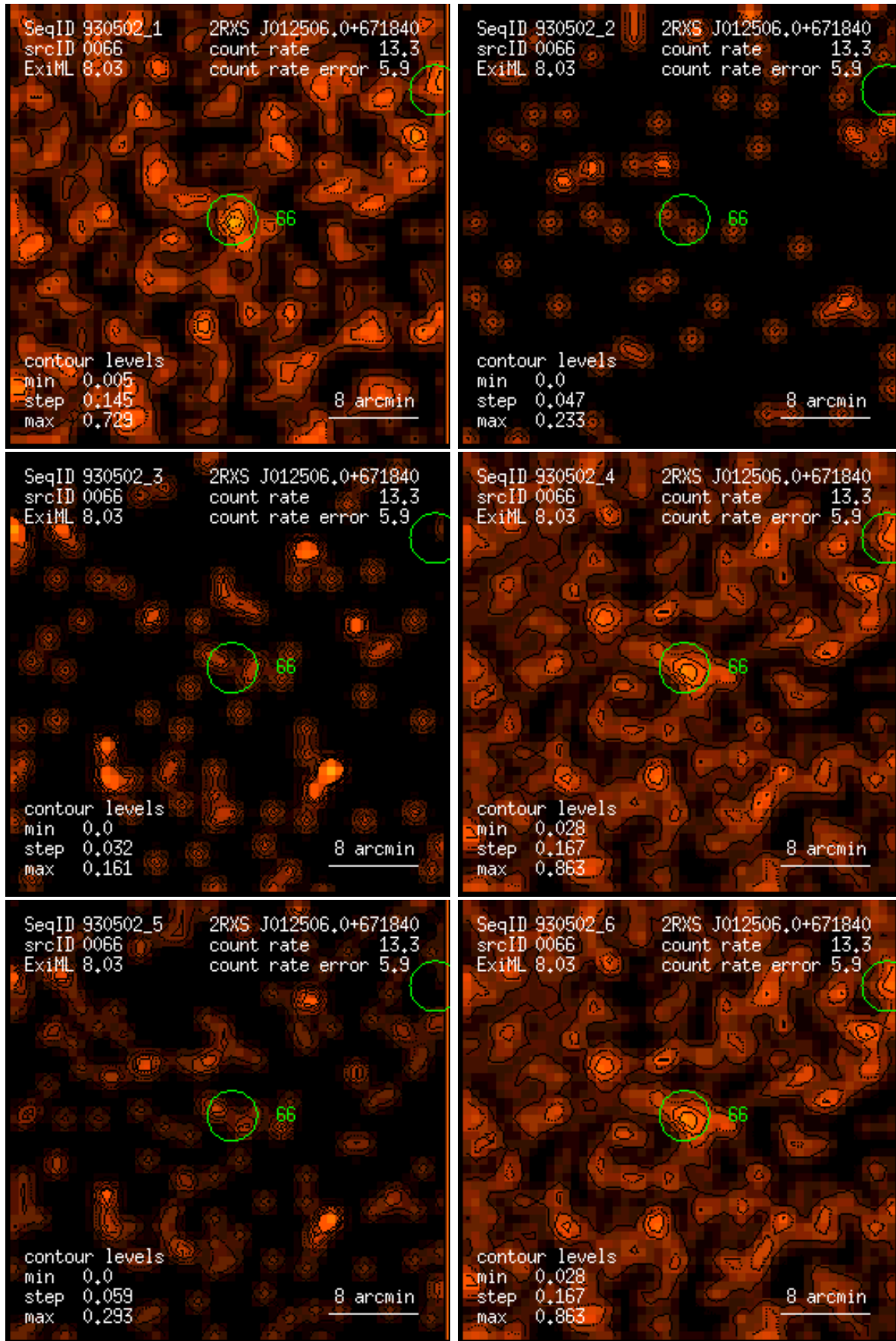
Figure 66: RASS 930502: detection 0066: band rate images, Gaussian filter: (1) PSPC channels 11 – 41, (2) 52 – 90, (3) 91 – 201, (4) 11 – 235, (5) 52 – 201, (6) 11 – 201. Broad band rates in counts/ks. Band rate contour levels in counts/ks/arcmin 2 .
